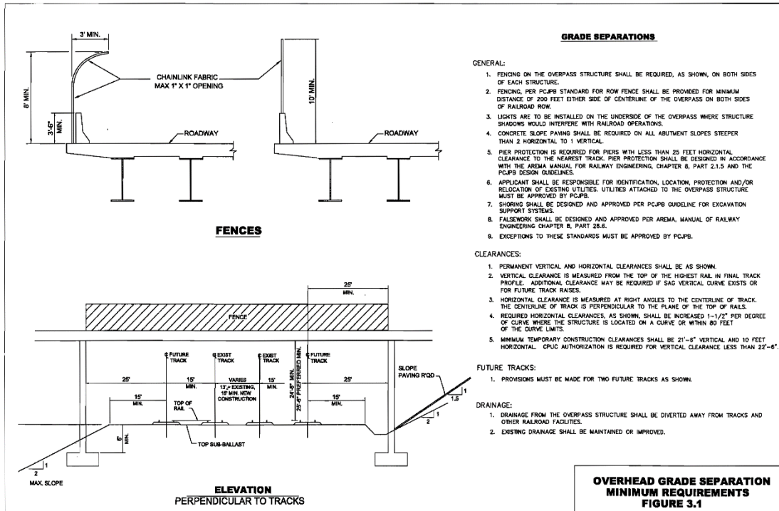
Figure 5-3 Caltrain Overhead Grade Separation Minimum Requirements
