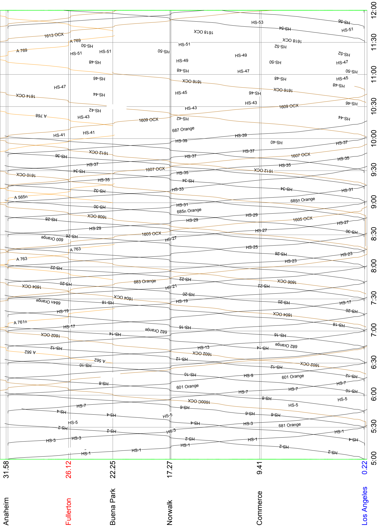
Figure 7 - LOSSAN Corridor Model Case 3 (HSR-OC Line) AM - Three and Two (with Shared Use)
