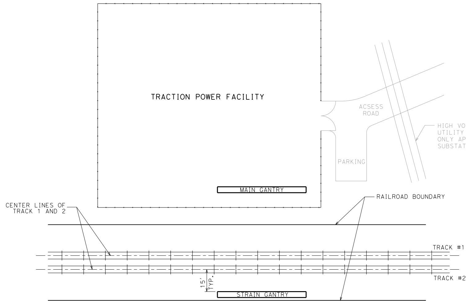
ALTERNATIVE #1: TPF LOCATED ADJACENT TO RAILROAD ROW
