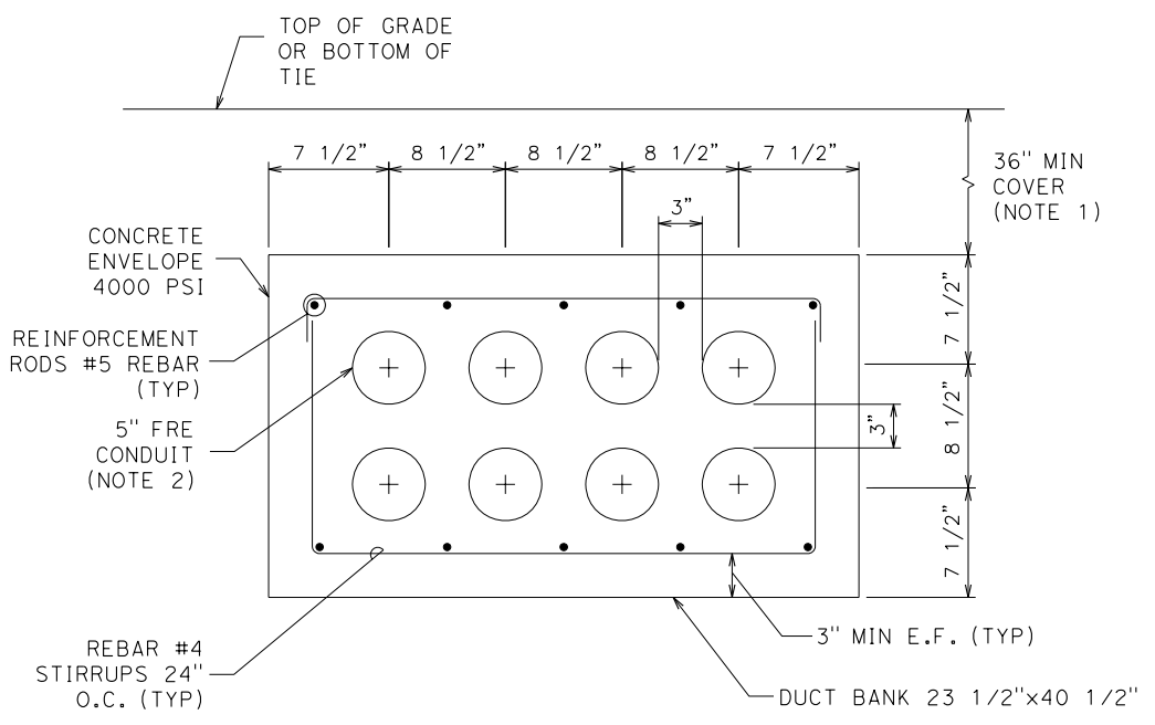
8-WAY DUCT BANK D - DETAIL SCALE: NTS
