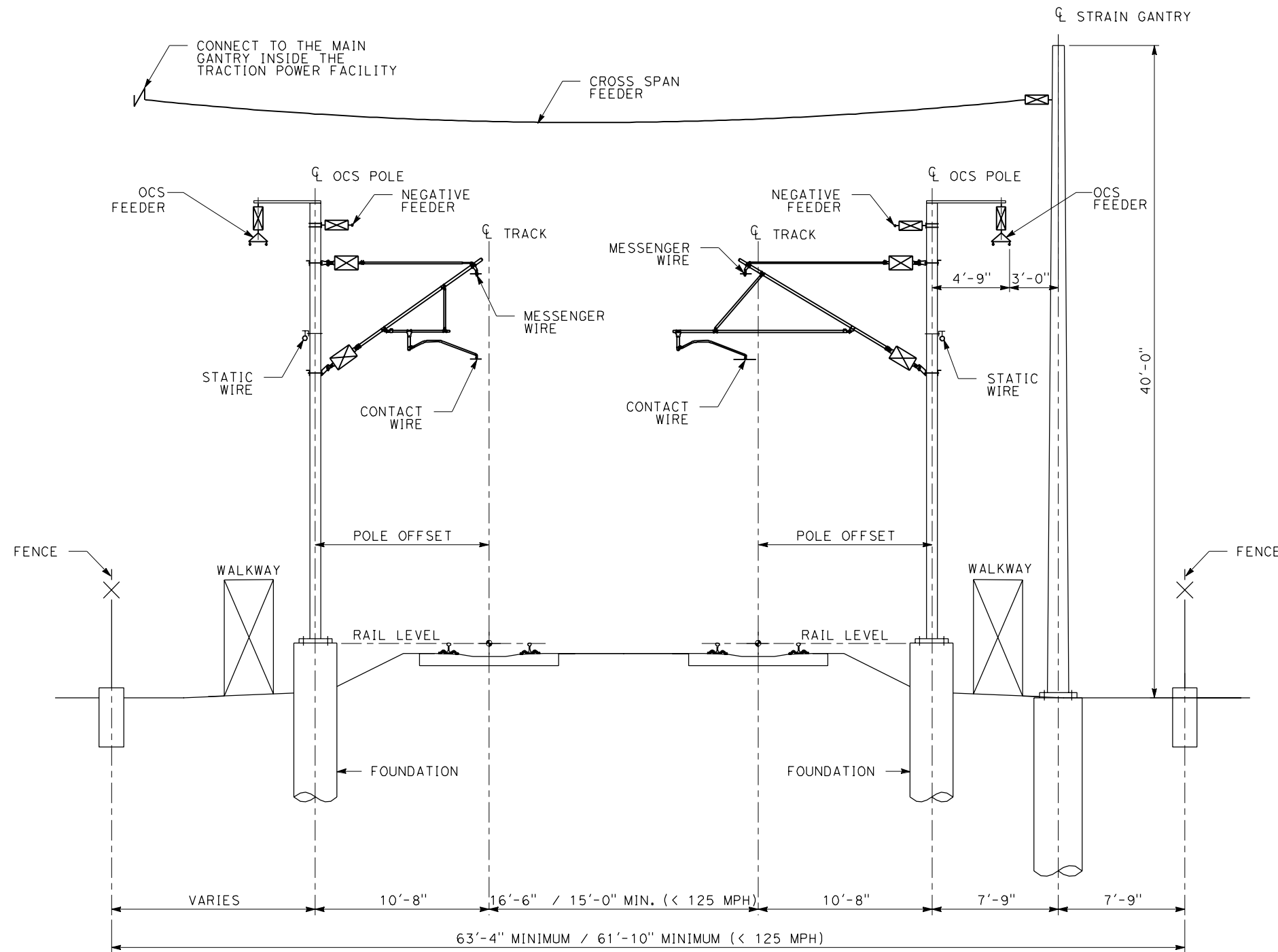
TYPICAL CATENARY FEEDING GANTRY ARRANGEMENT- TPF LOCATED CLOSE TO RAILROAD ROW
