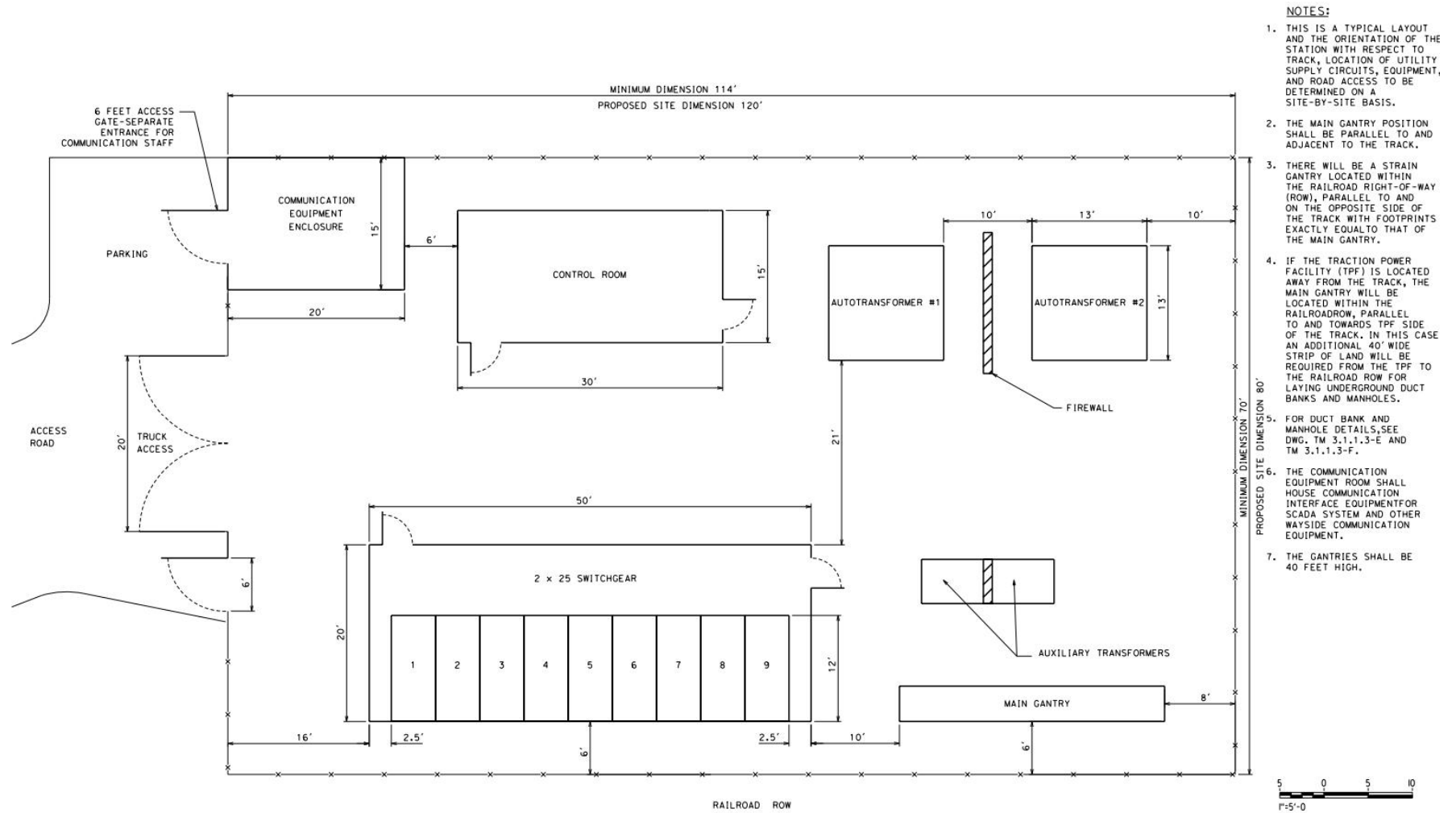
CONCEPTUAL LAYOUT PARALLELING STATION WITH 2 AUTOTRANSFORMERS - FIGURE 4
