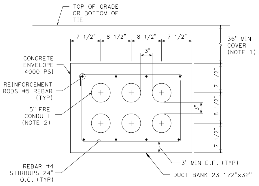
6-WAY DUCT BANK E - DETAIL SCALE: NTS
