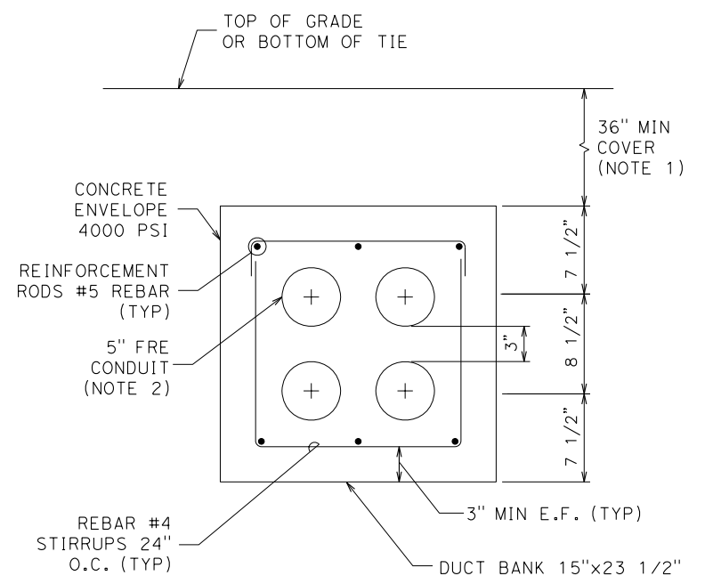
4-WAY DUCT BANK C - DETAIL SCALE: NTS
