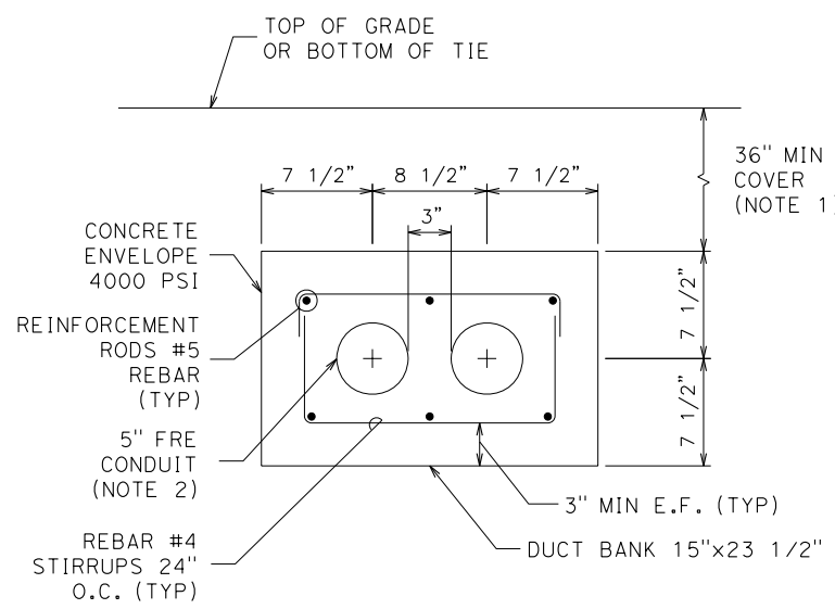
2-WAY DUCT BANK A - DETAIL SCALE: NTS
