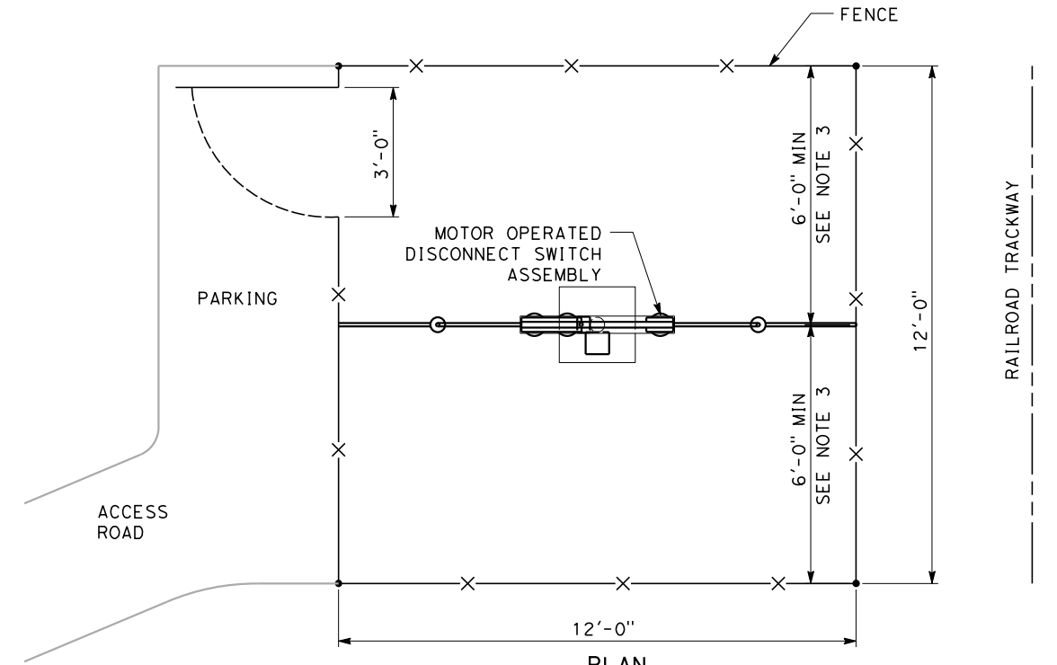
MOTOR OPERATED DISCONNECT SWITCH ASSEMBLY SPACE ARRANGEMENT CABLE DETAILS OMITTED FOR CLARITY (SEE NOTE 3)
