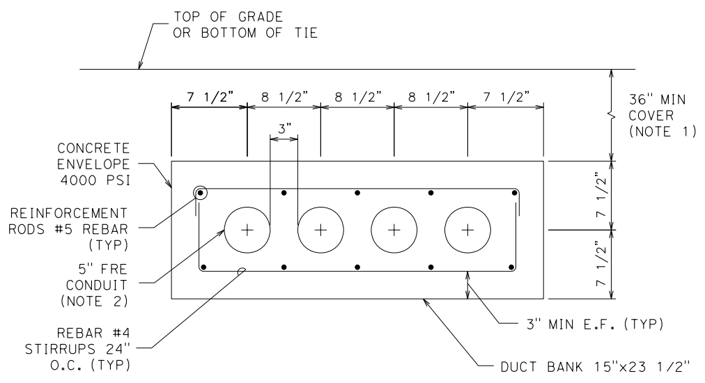
4-WAY DUCT BANK B - DETAIL SCALE: NTS
