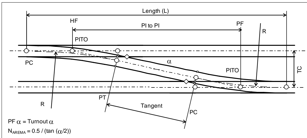
Figure 6.3.1: Crossovers
