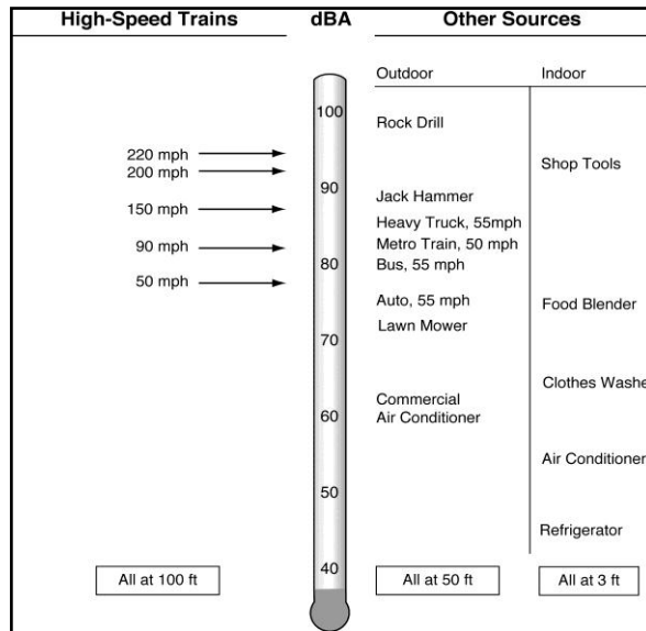
Figure 3.4-1 Typical L max noise levels
