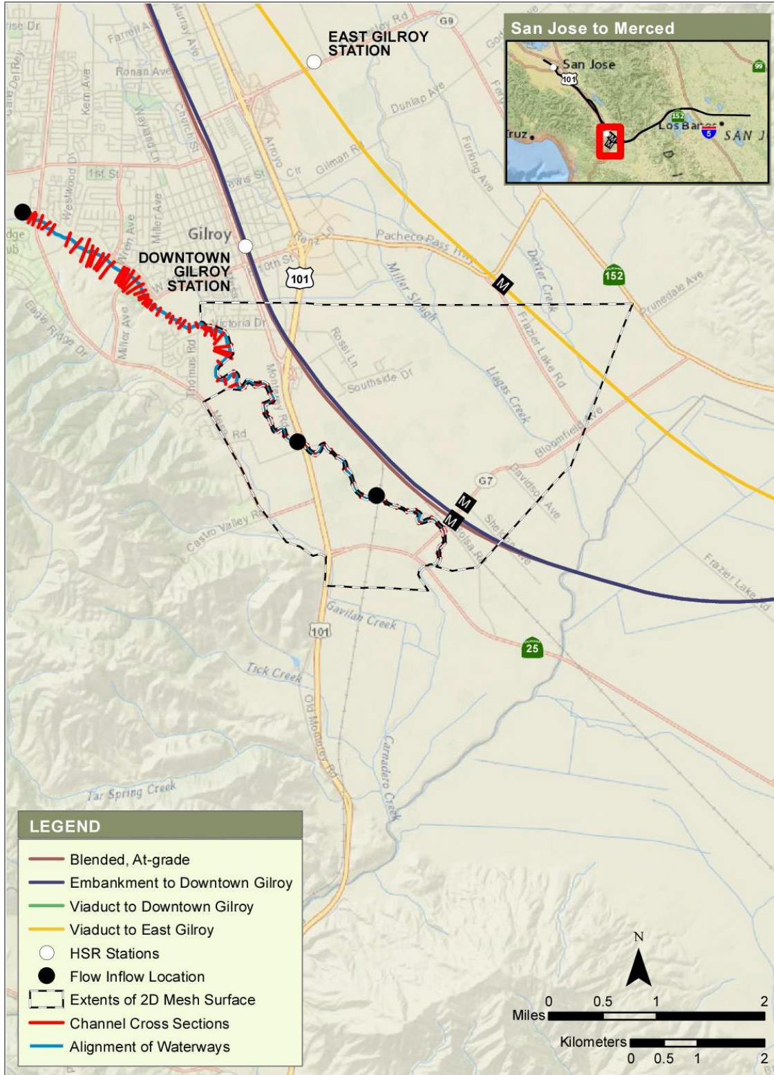
Figure 4-32 Inflow Locations in the Hydraulic Model of Uvas-Carnadero Creek
