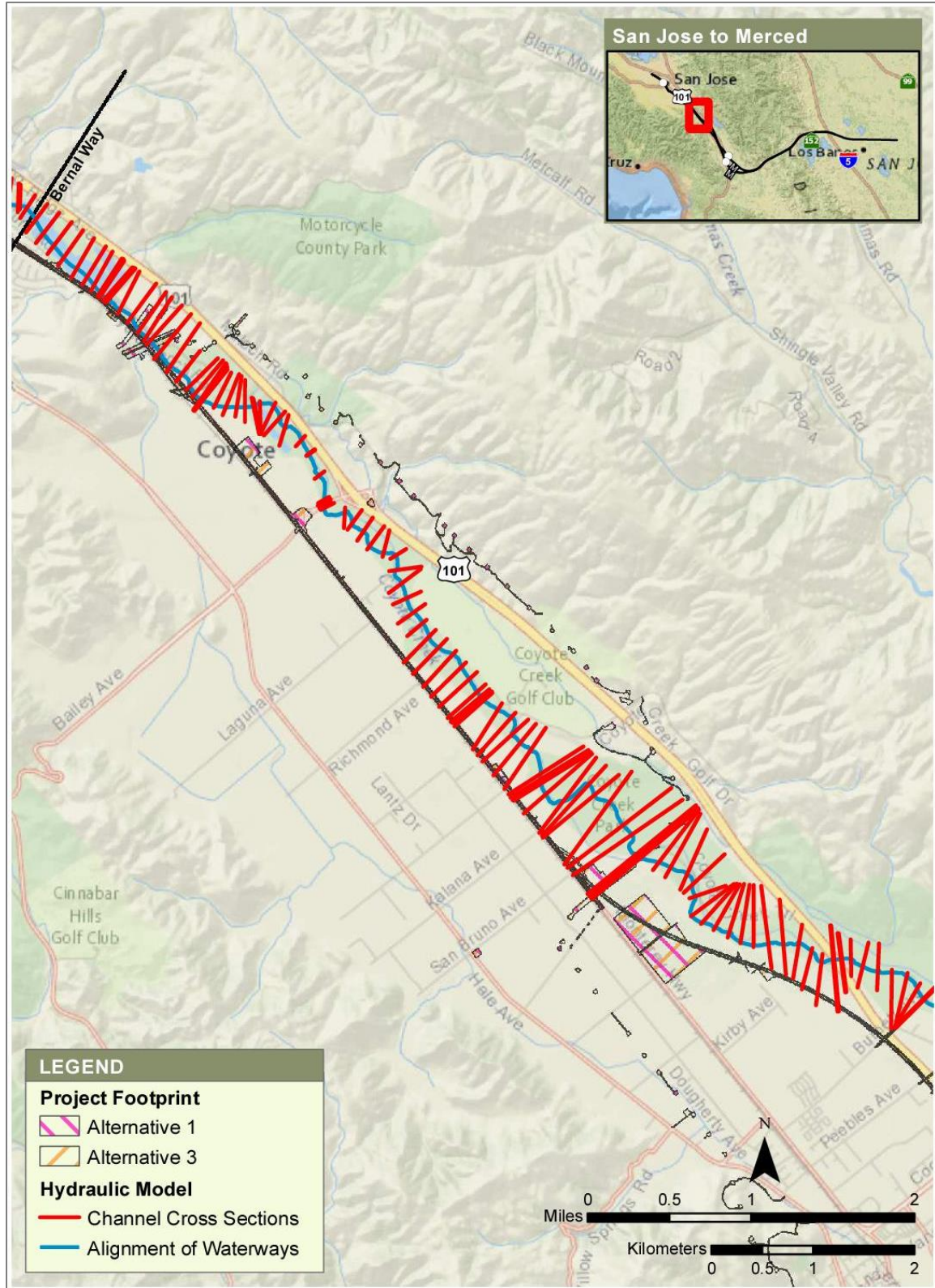
Figure 3-6 Coyote Creek, Plan View of SCVWD Hydraulic Model with Project Footprint for Alternatives 1 and 3
