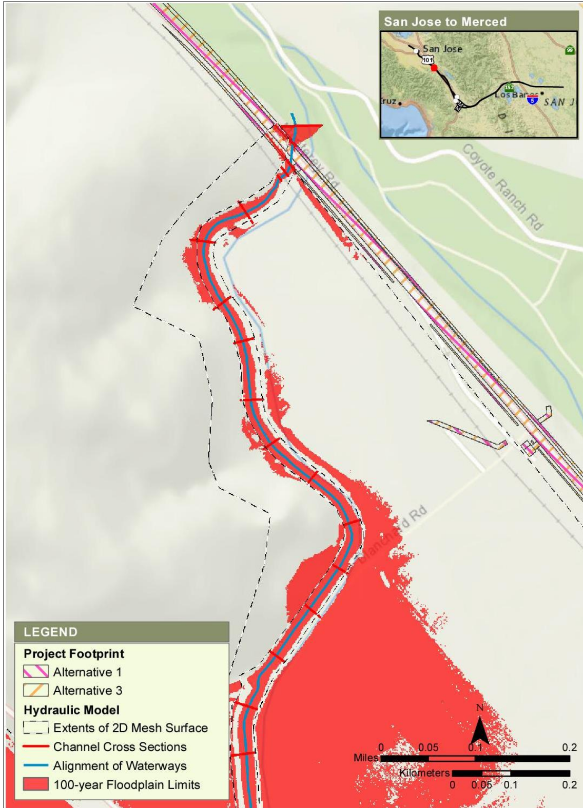
Figure 4-28 Fisher Creek 100-Year Floodplain from Hydraulic Analysis, Alternatives 1 and 3
