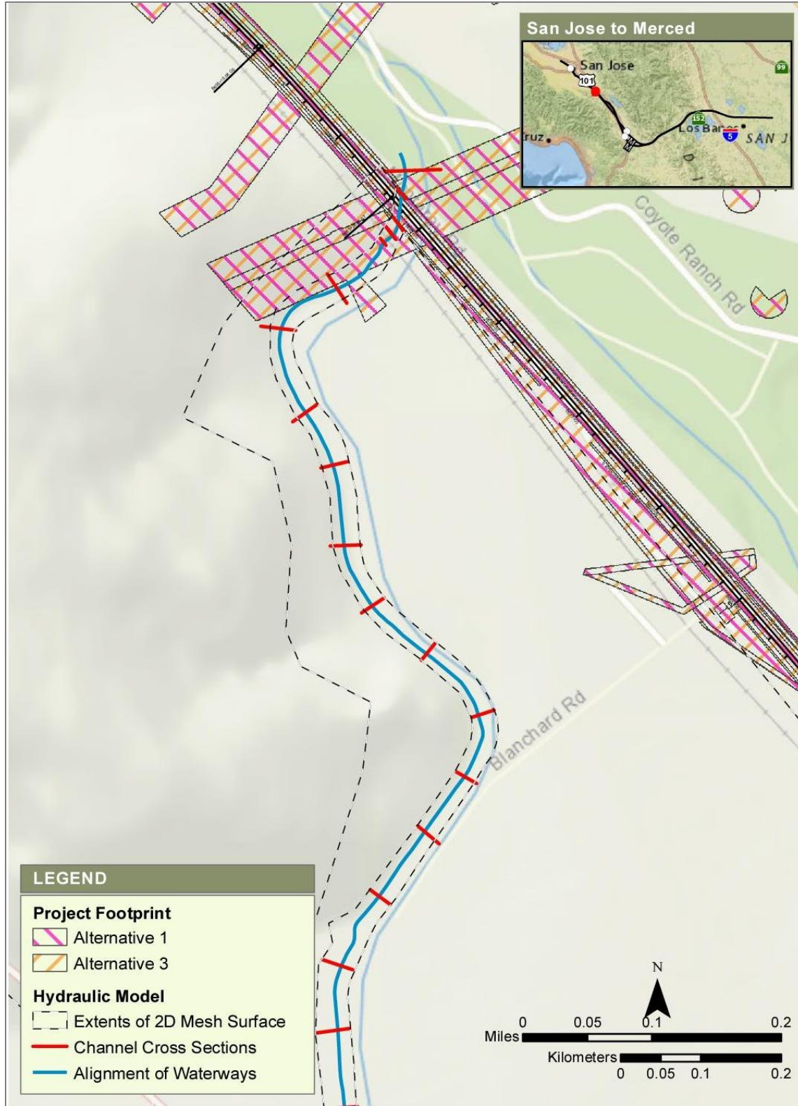
Figure 4-23 Fisher Creek, Plan View of SCVWD Hydraulic Model with Project Footprints for Alternatives 1 and 3
