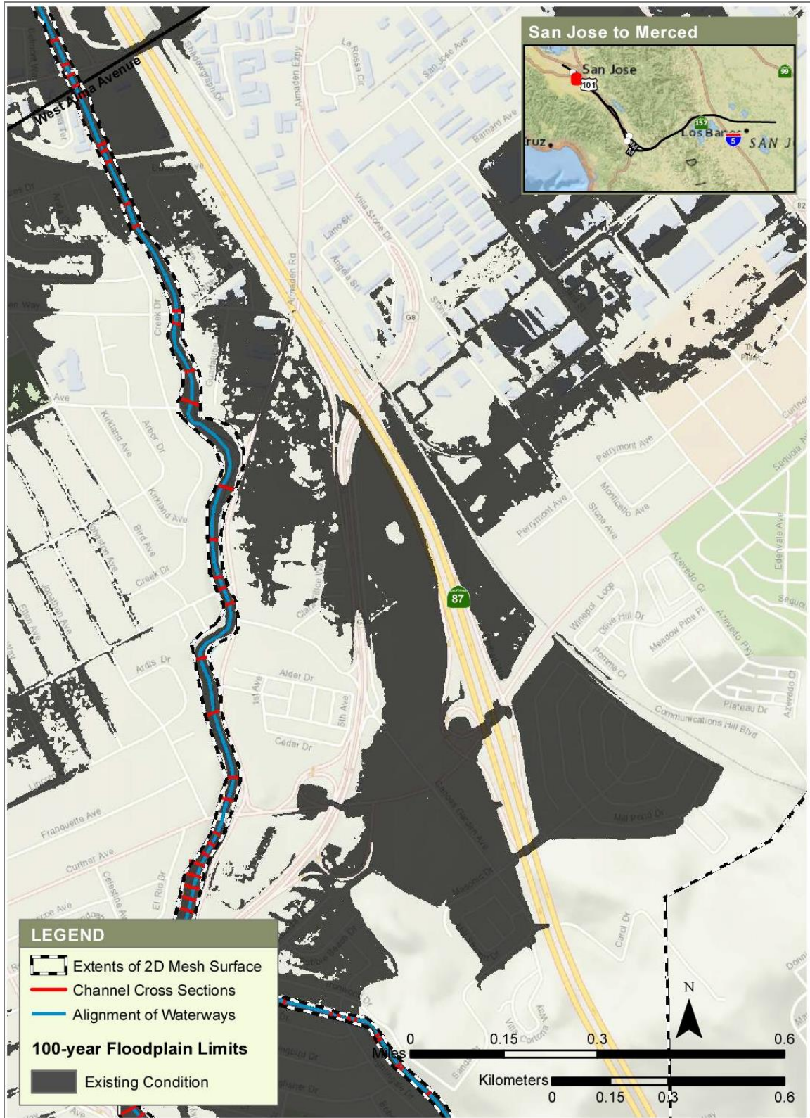
Figure 4-17 100-Year Floodplain at Almaden-Curtner Area from Hydraulic Analysis, Existing Condition
