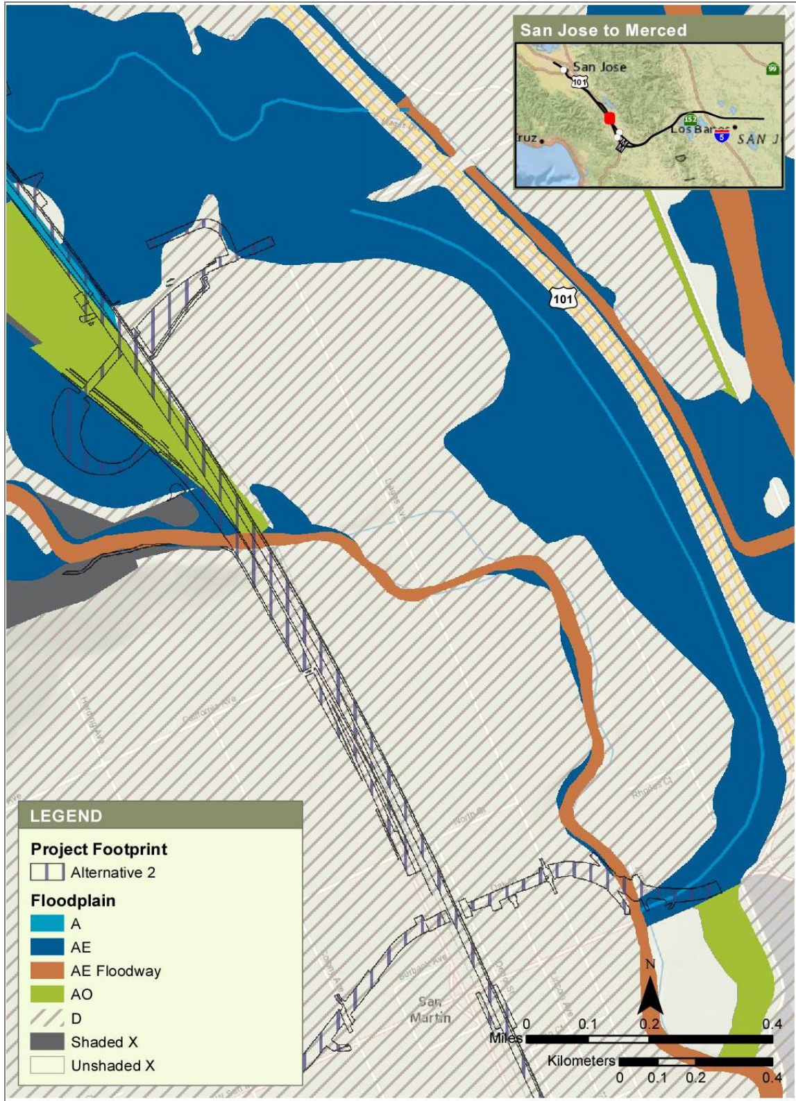
Figure 3-33 West Little Llagas Creek Middle Avenue Overflow, Plan View of FEMA Effective Hydraulic Model with Project Footprint for Alternative 2
