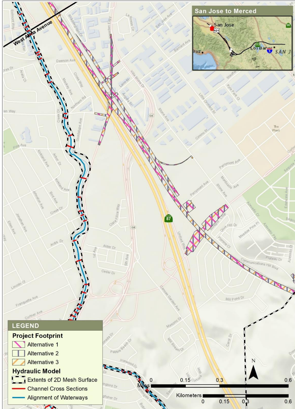
Figure 4-10 Guadalupe River, Plan View of SCVWD Hydraulic Model at Almaden-Curtner Area with Project Footprint for Alternatives 1, 2, and 3
