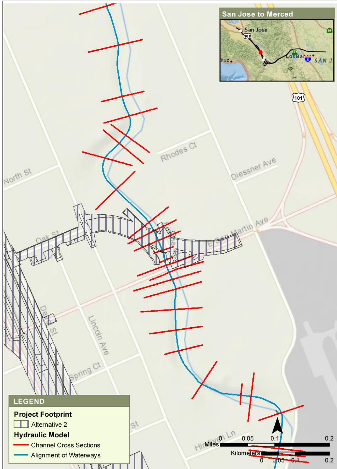
Figure 3-32 Llagas Creek (At East San Martin Avenue), Plan View of SCVWD Hydraulic Model with Project Footprint for Alternative 2
