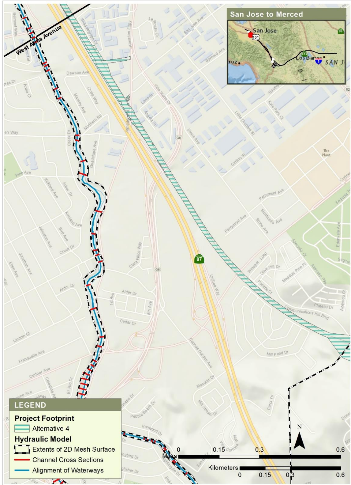
Figure 4-11 Guadalupe River, Plan View of SCVWD Hydraulic Model at Almaden-Curtner Area with Project Footprint for Alternative 4
