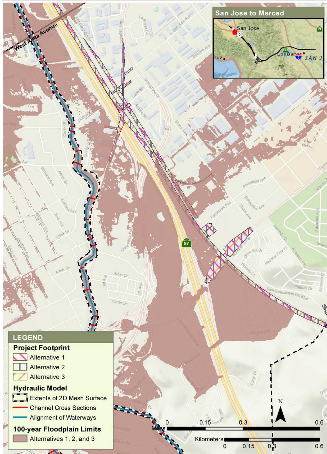
Figure 4-20 100-Year Floodplain at Almaden-Curtner Area from Hydraulic Analysis, Alternatives 1, 2, and 3 with Floodwall and Equalizer Culverts
