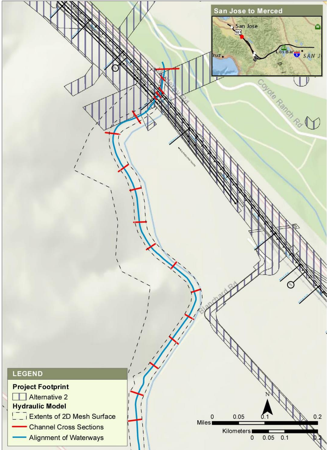
Figure 4-24 Fisher Creek, Plan View of SCVWD Hydraulic Model with Project Footprint for Alternative 2
