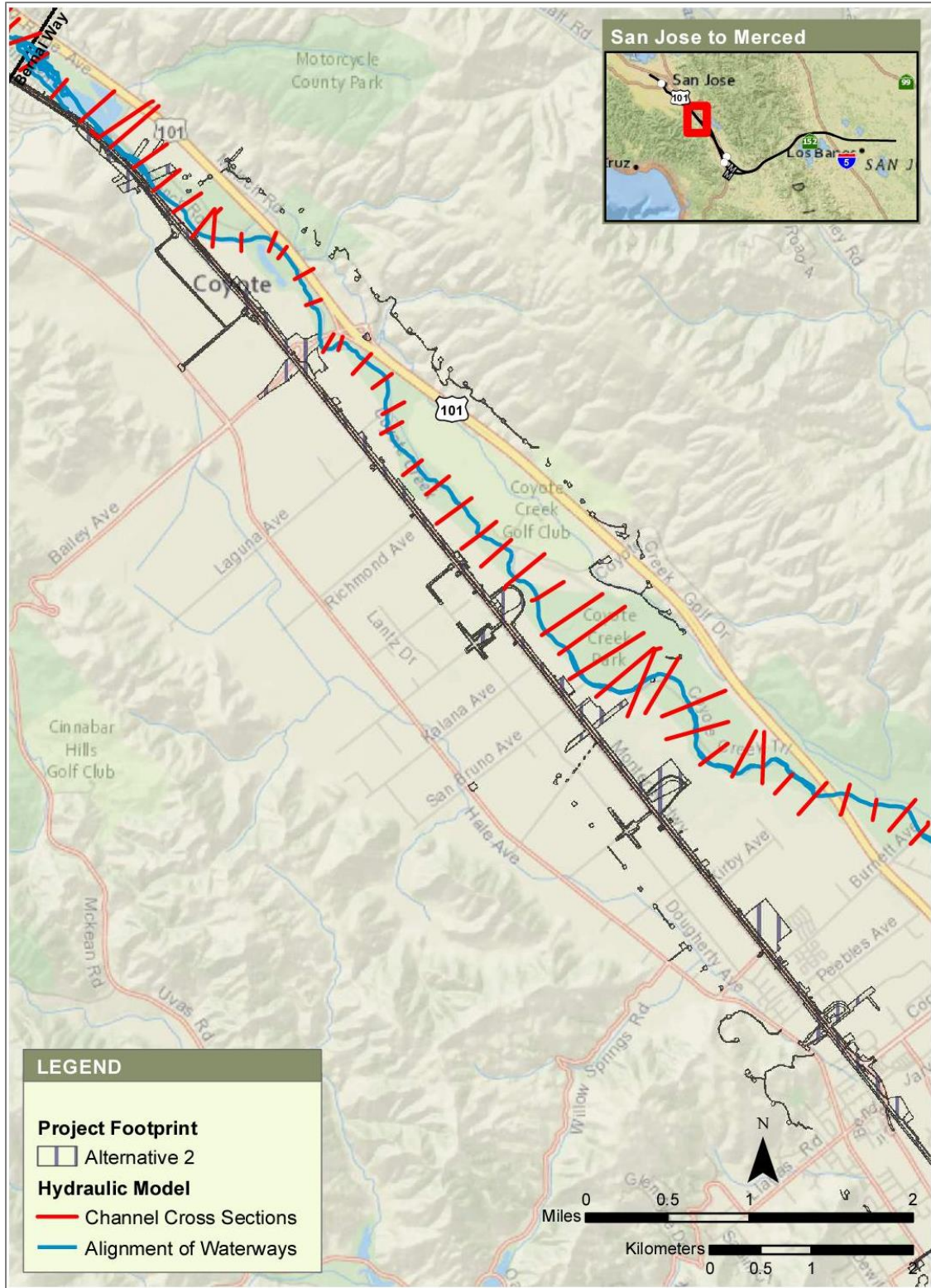
Figure 3-4 Coyote Creek, Plan View of FEMA Effective Hydraulic Model with Project Footprint for Alternative 2
