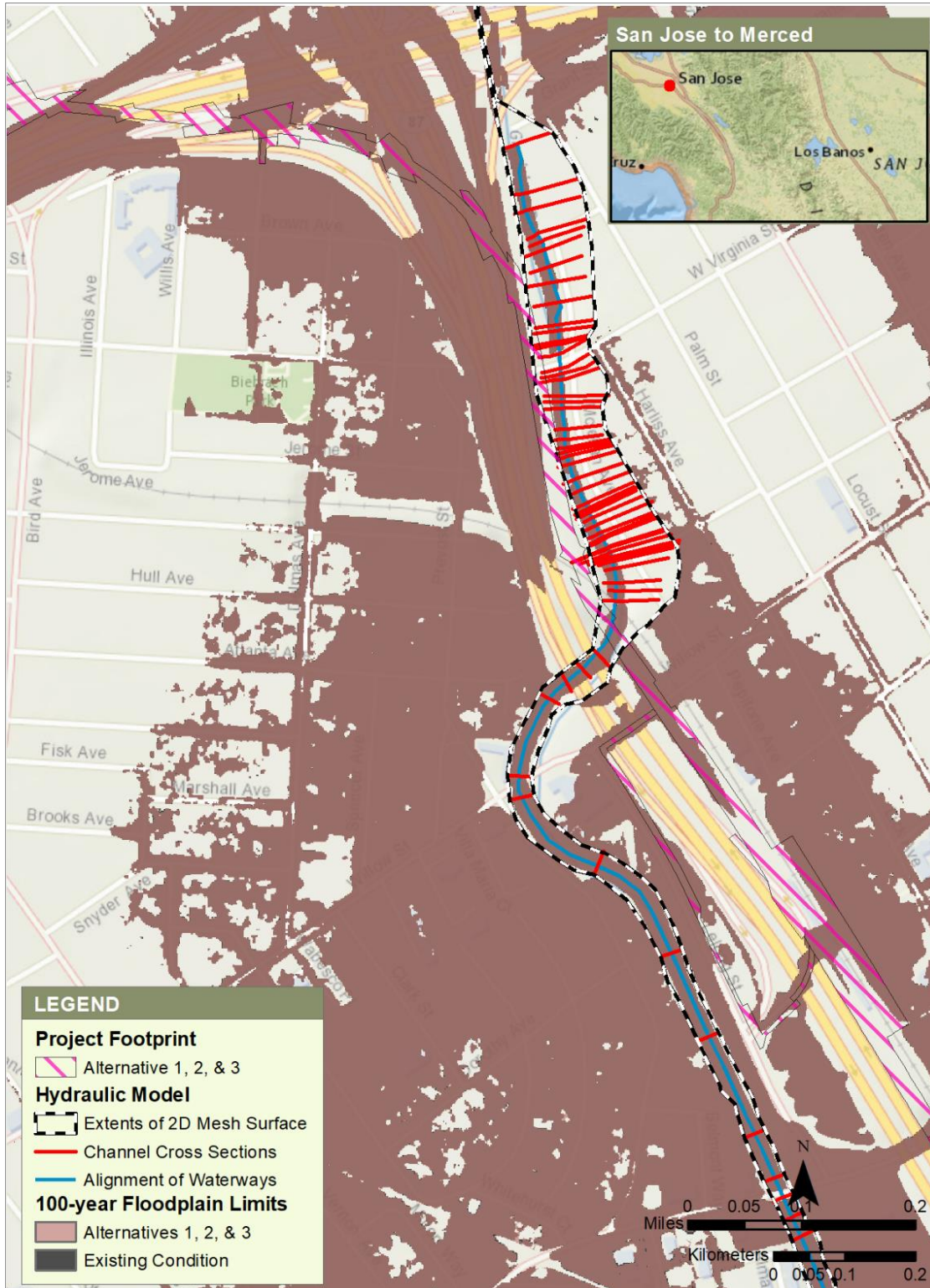
Figure 4-13 Guadalupe River, 100-Year Floodplain Footprints from Hydraulic Analysis for Existing Condition and Alternatives 1, 2, and 3
