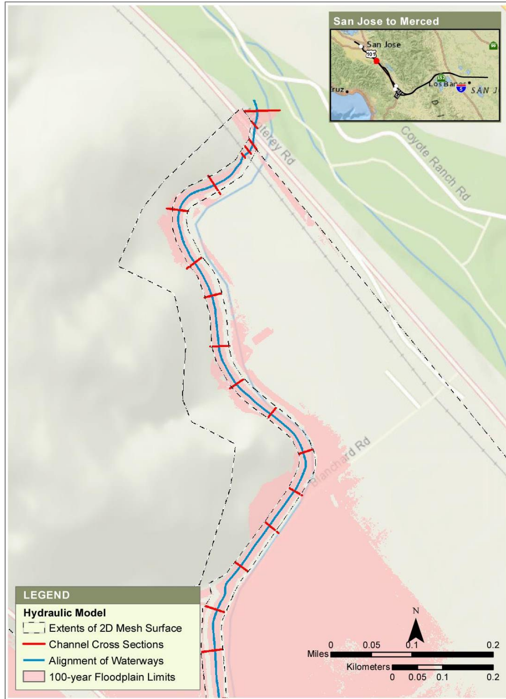
Figure 4-27 Fisher Creek 100-Year Floodplain from Hydraulic Analysis, Existing Condition
