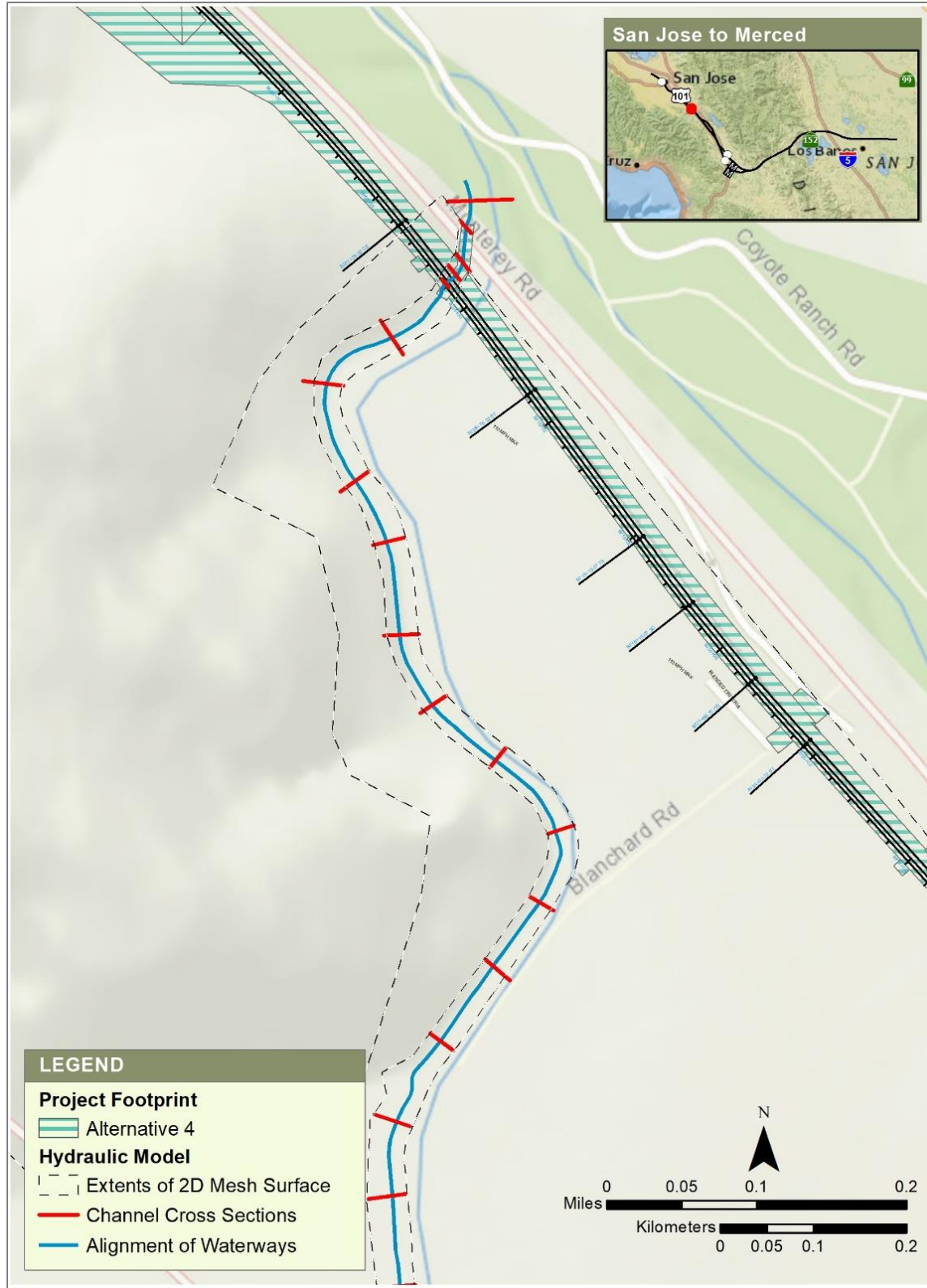
Figure 4-25 Fisher Creek, Plan View of SCVWD Hydraulic Model with Project Footprint for Alternative 4
