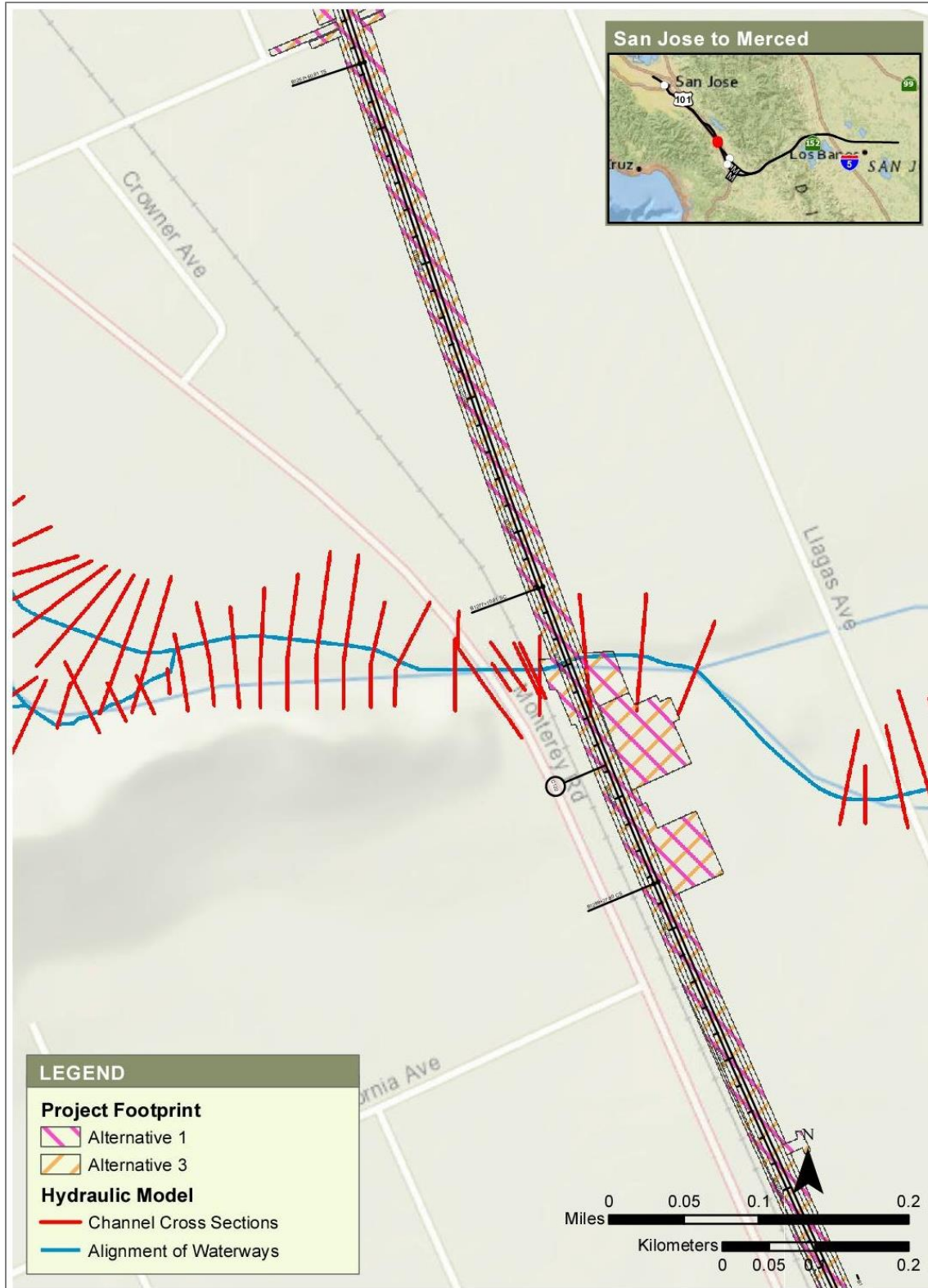
Figure 3-26 Llagas Creek (near San Martin), Plan View of SCVWD Model at Proposed HSR Crossing, Alternatives 1 and 3
