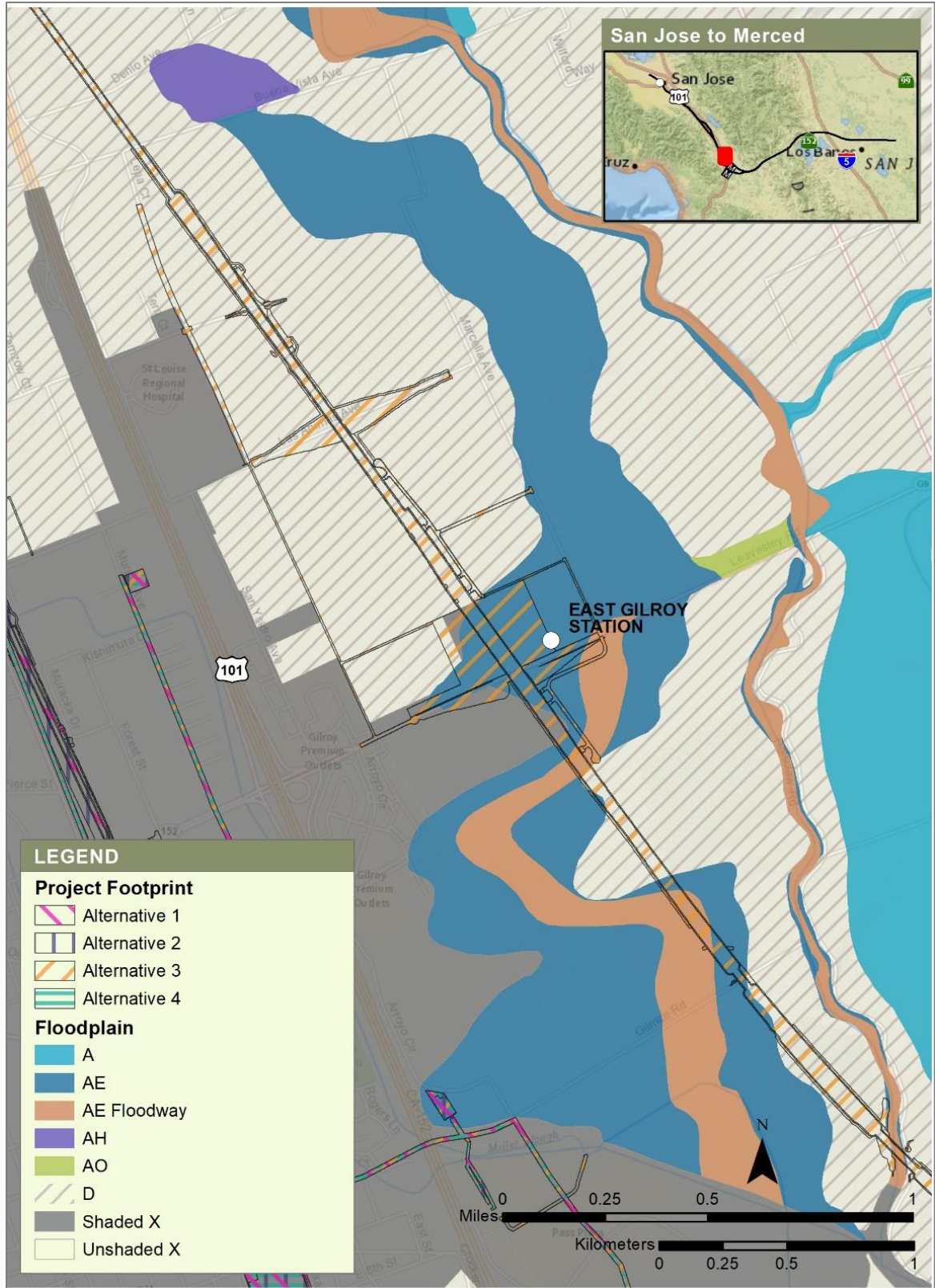
Figure 3-43 Llagas Overbank, FEMA FIRM Zoomed to Project Location
