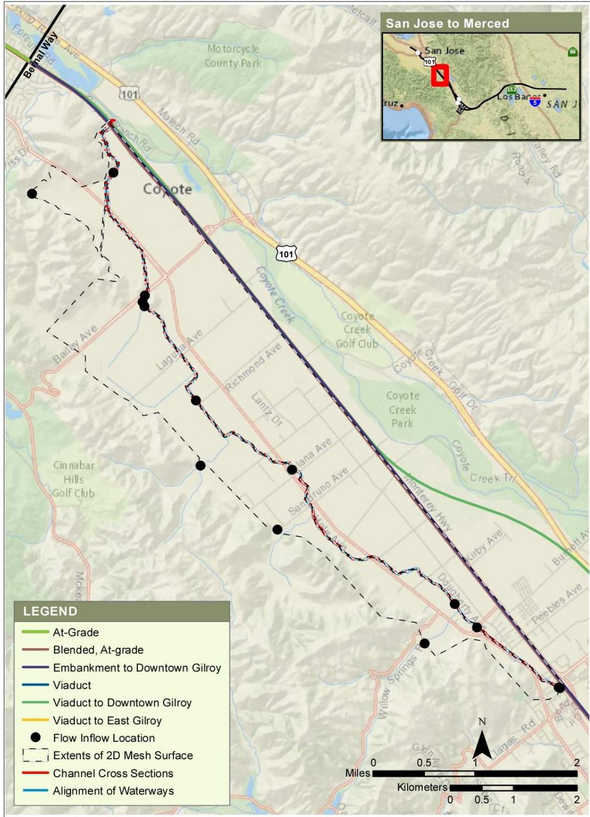
Figure 4-26 Inflow Locations in the Fisher Creek Hydraulic Model
