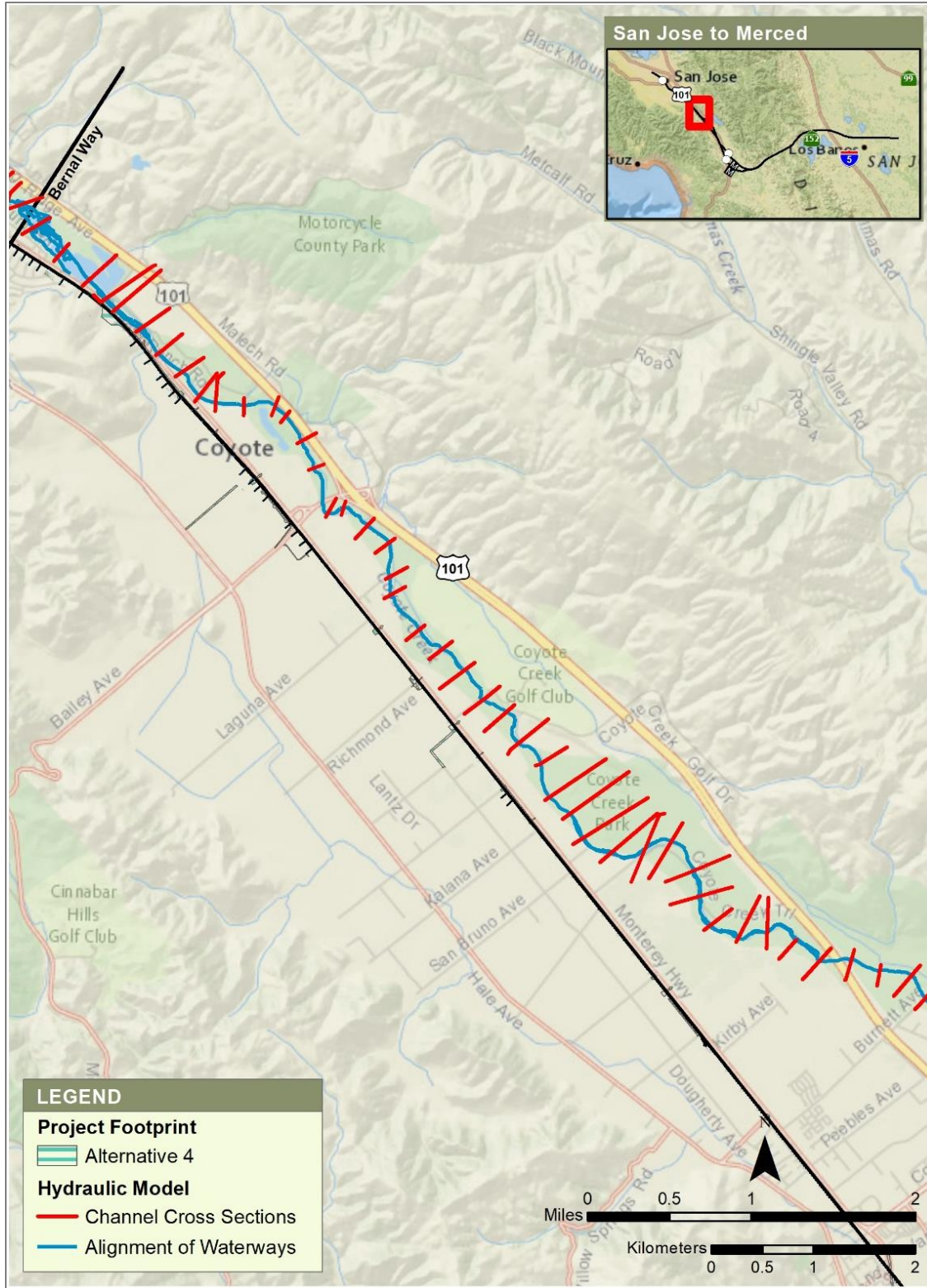
Figure 3-5 Coyote Creek, Plan View of FEMA Effective Hydraulic Model with Project Footprint for Alternative 4
