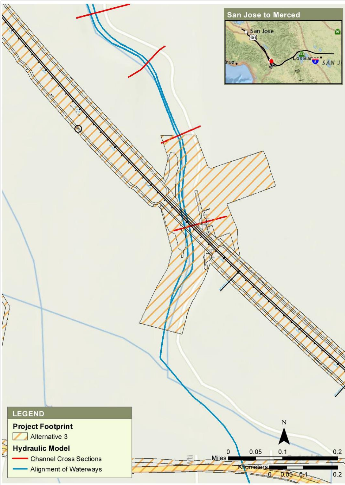
Figure 3-40 Llagas Creek (East of Gilroy), FEMA Hydraulic Model at Project Location
