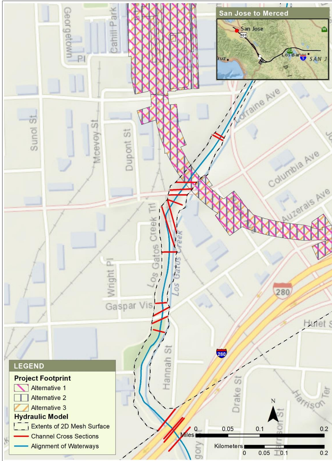
Figure 4-2 Los Gatos Creek, Plan View of SCVWD Hydraulic Model with Project Footprint for Alternatives 1, 2, and 3
