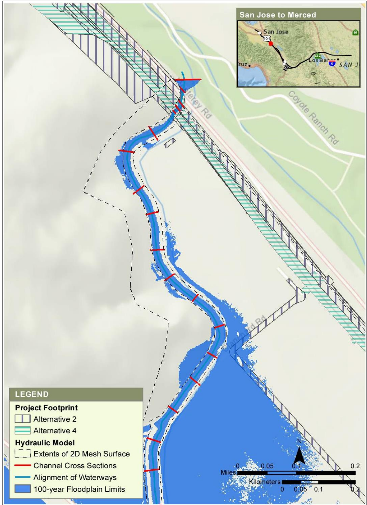
Figure 4-29 Fisher Creek 100-Year Floodplains from Hydraulic Analysis, Alternatives 2 and 4
