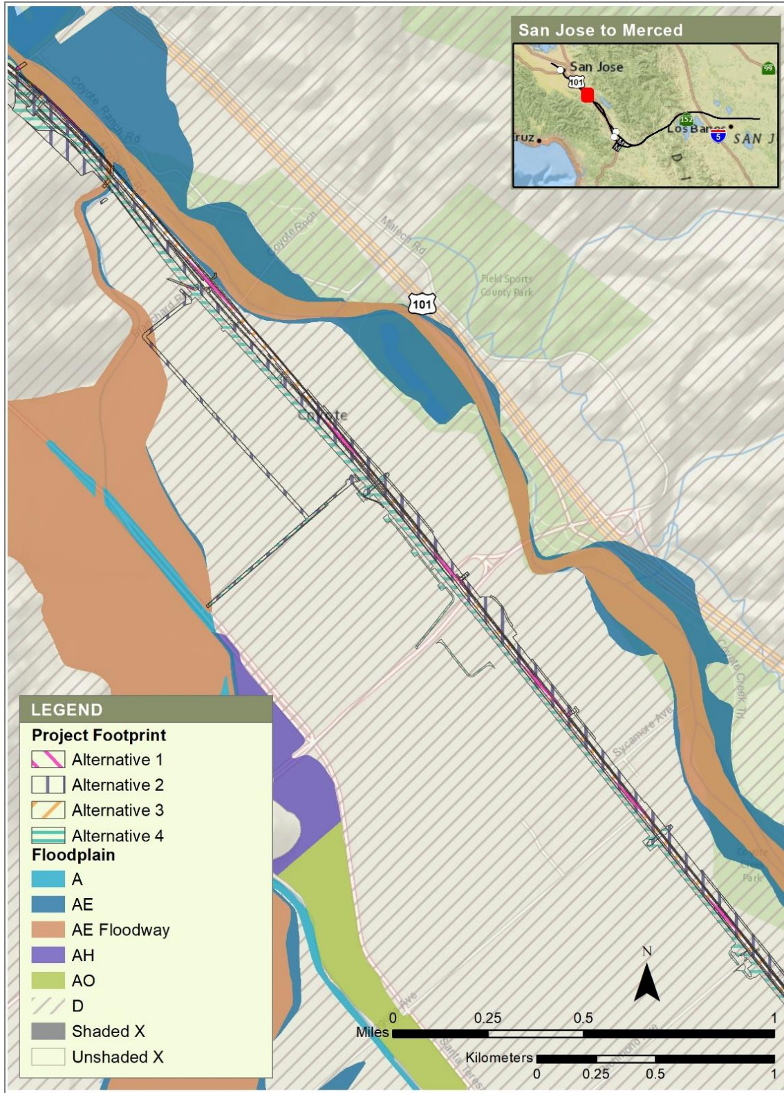
Figure 3-1 Coyote Creek, FEMA FIRM Overlay with Project Footprints for Alternatives 1, 2, 3, and 4, Page 1/2
