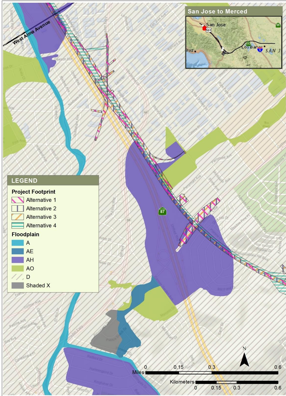
Figure 4-7 Guadalupe River, FEMA FIRM Overlay at Almaden-Curtner Area with Project Footprints for Alternatives 1, 2, 3, and 4
