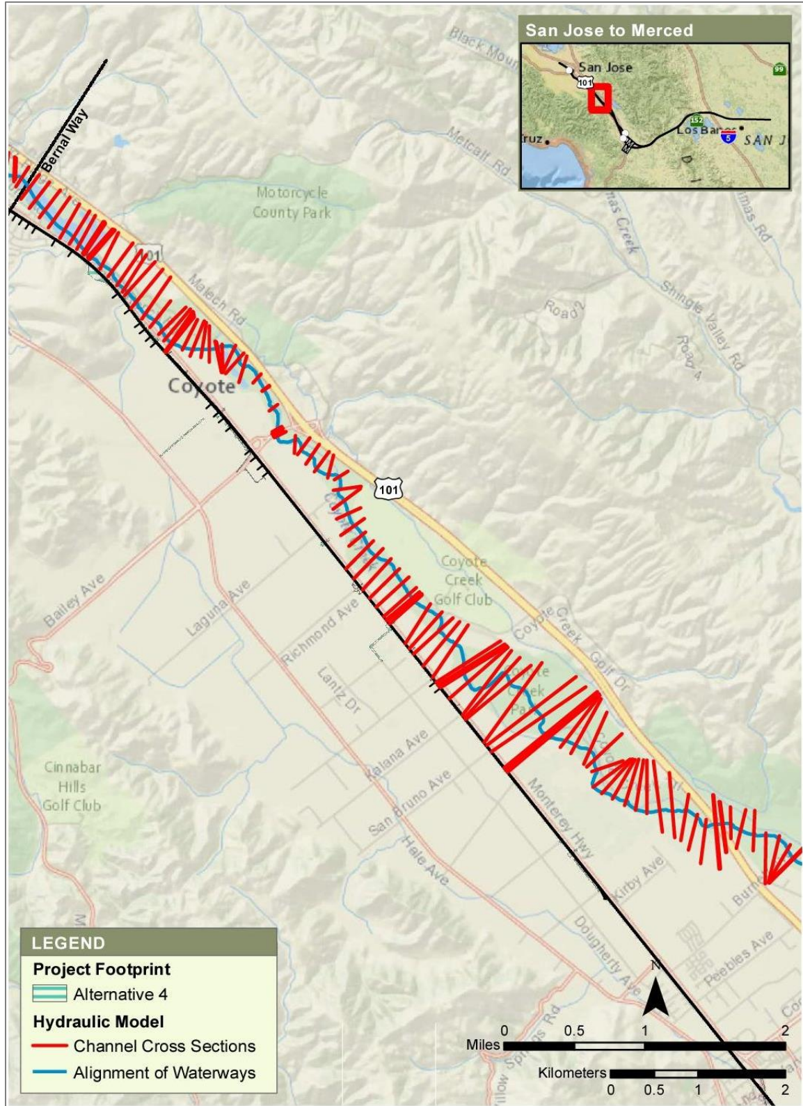
Figure 3-8 Coyote Creek, Plan View of SCVWD Hydraulic Model with Project Footprint for Alternative 4
