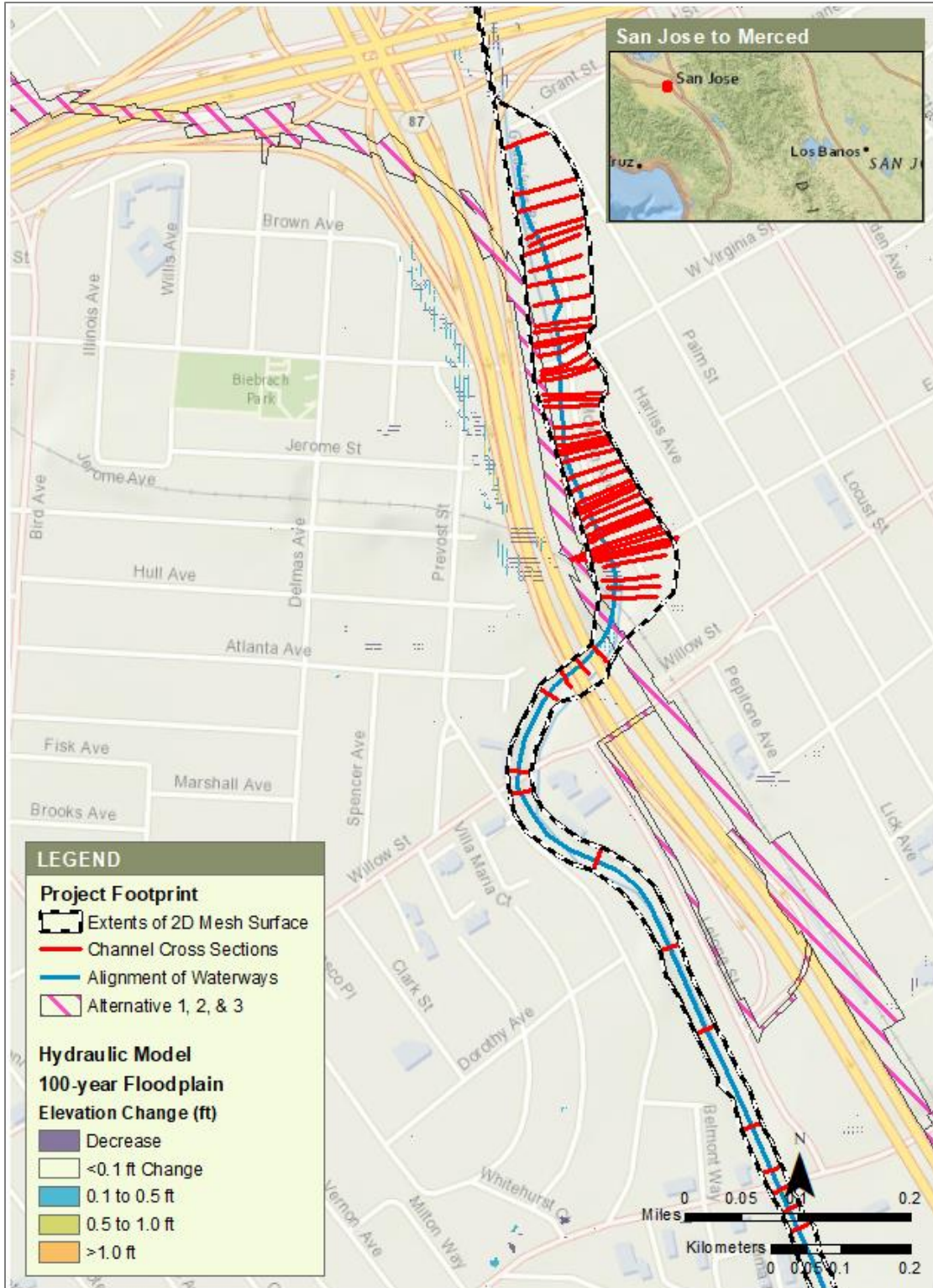
Figure 4-15 Guadalupe River, 100-Year Floodplain Elevation Change From Existing Condition to Alternatives 1, 2, and 3
