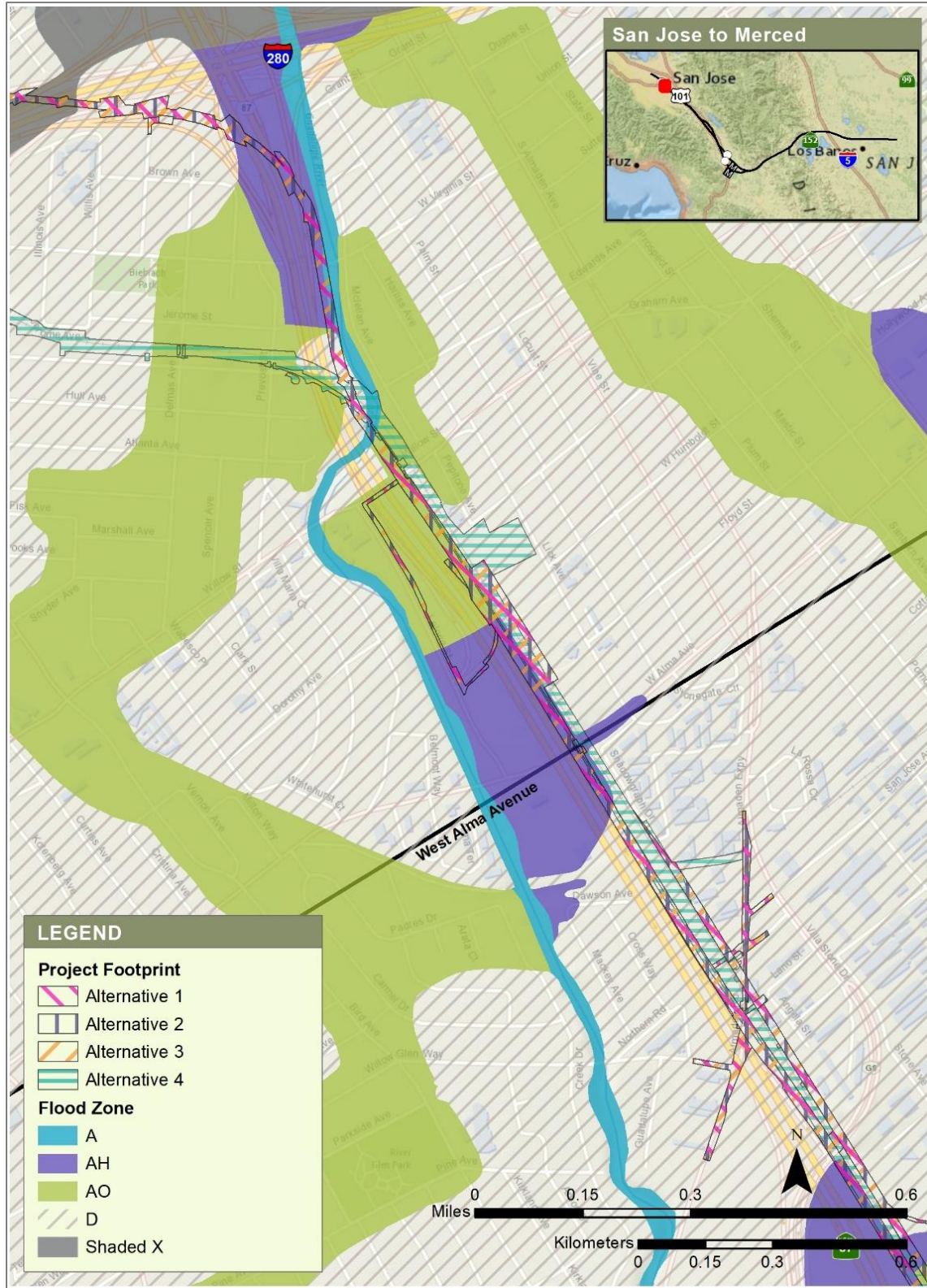
Figure 4-6 Guadalupe River, FEMA FIRM Overlay at Guadalupe River Bridge with Project Footprints for Alternatives 1, 2, 3, and 4
