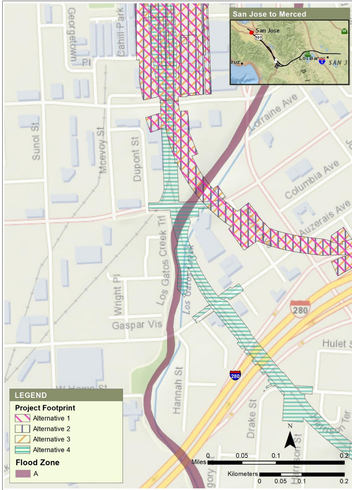
Figure 4-1 Los Gatos Creek, FEMA FIRM Overlay with Project Footprints for Alternatives 1, 2, 3, and 4
