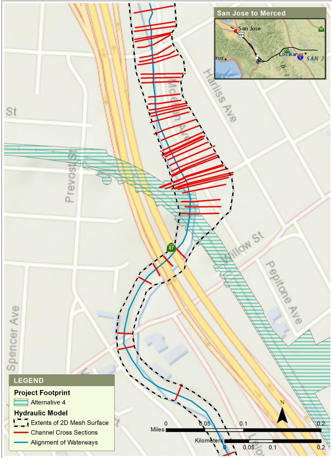
Figure 4-9 Guadalupe River, Plan View of SCVWD Hydraulic Model at Guadalupe River Mainline with Project Footprint for Alternative 4
