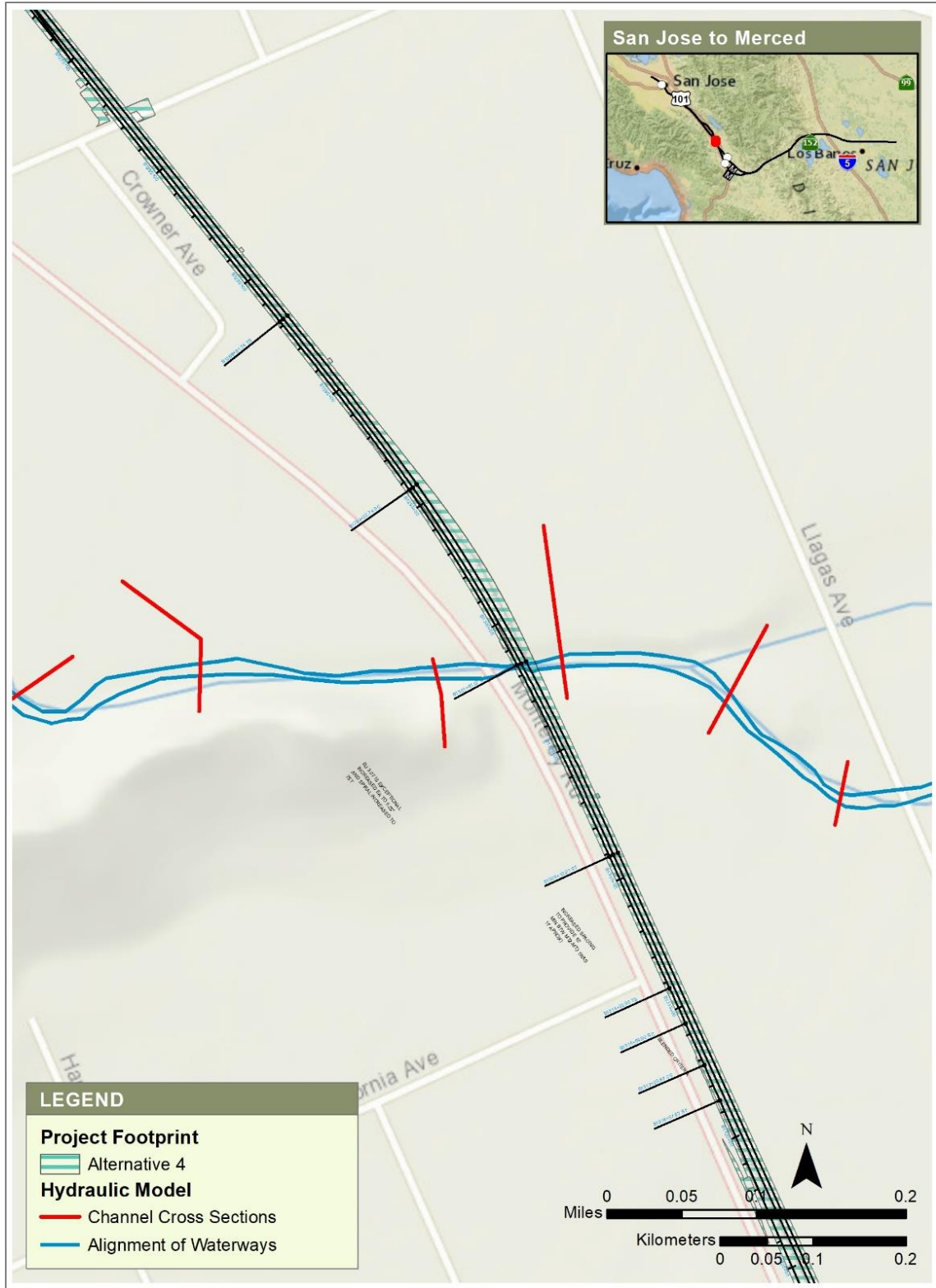
Figure 3-25 Llagas Creek (near San Martin), Plan View of FEMA Effective Hydraulic Model with Project Footprint for Alternative 4
