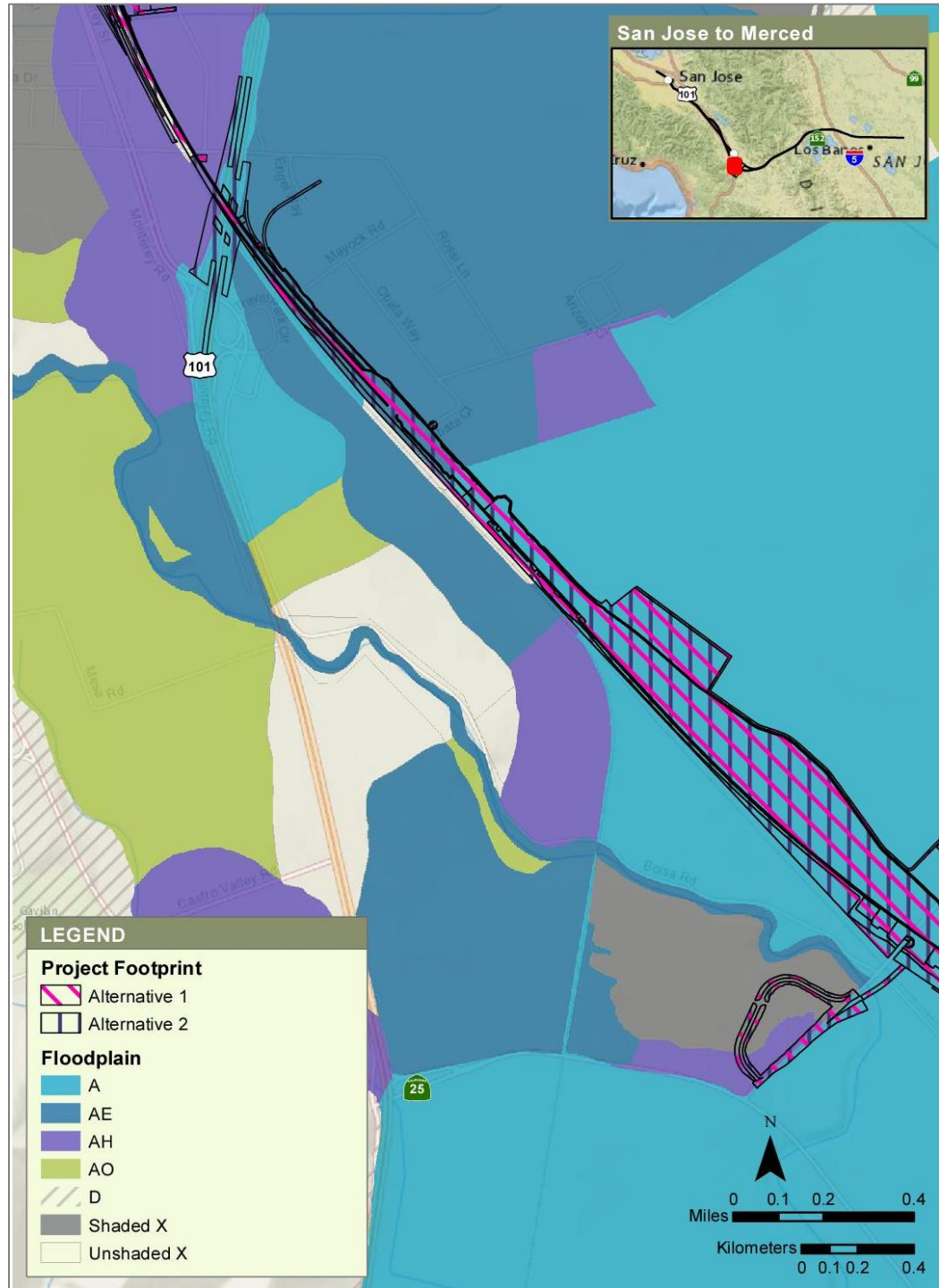
Figure 4-30 FEMA FIRM, Uvas-Carnadero Creek at Project Location with Project Footprints for Alternatives 1 and 2
