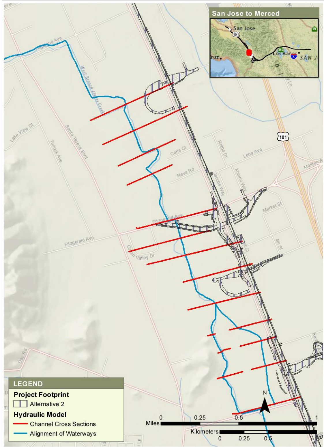
Figure 3-37 West Branch Llagas Creek, Plan View of FEMA Effective Hydraulic Model with Project Footprint for Alternative 2
