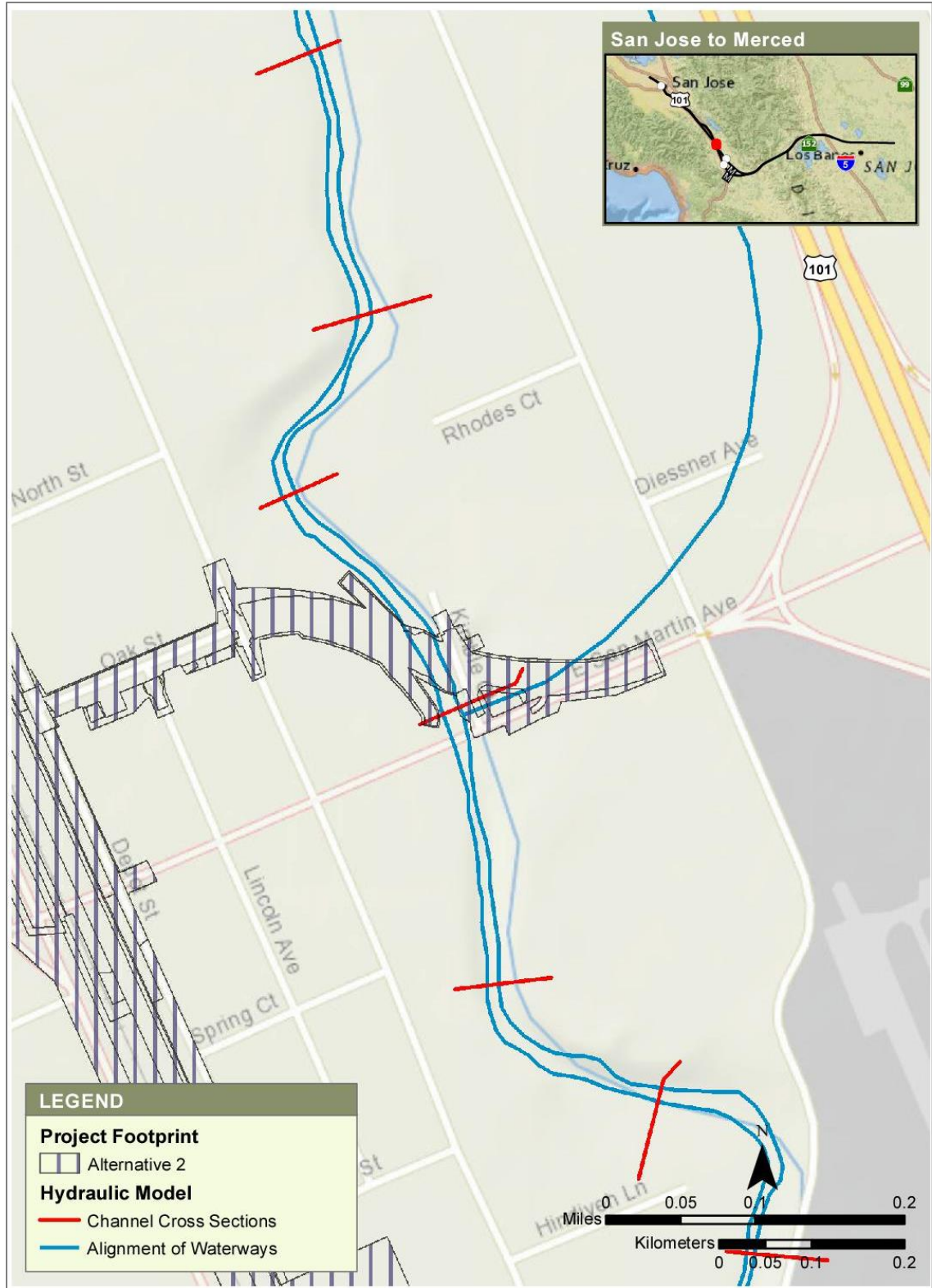
Figure 3-31 Llagas Creek (At East San Martin Avenue), Plan View of FEMA Effective Hydraulic Model with Project Footprint for Alternative 2
