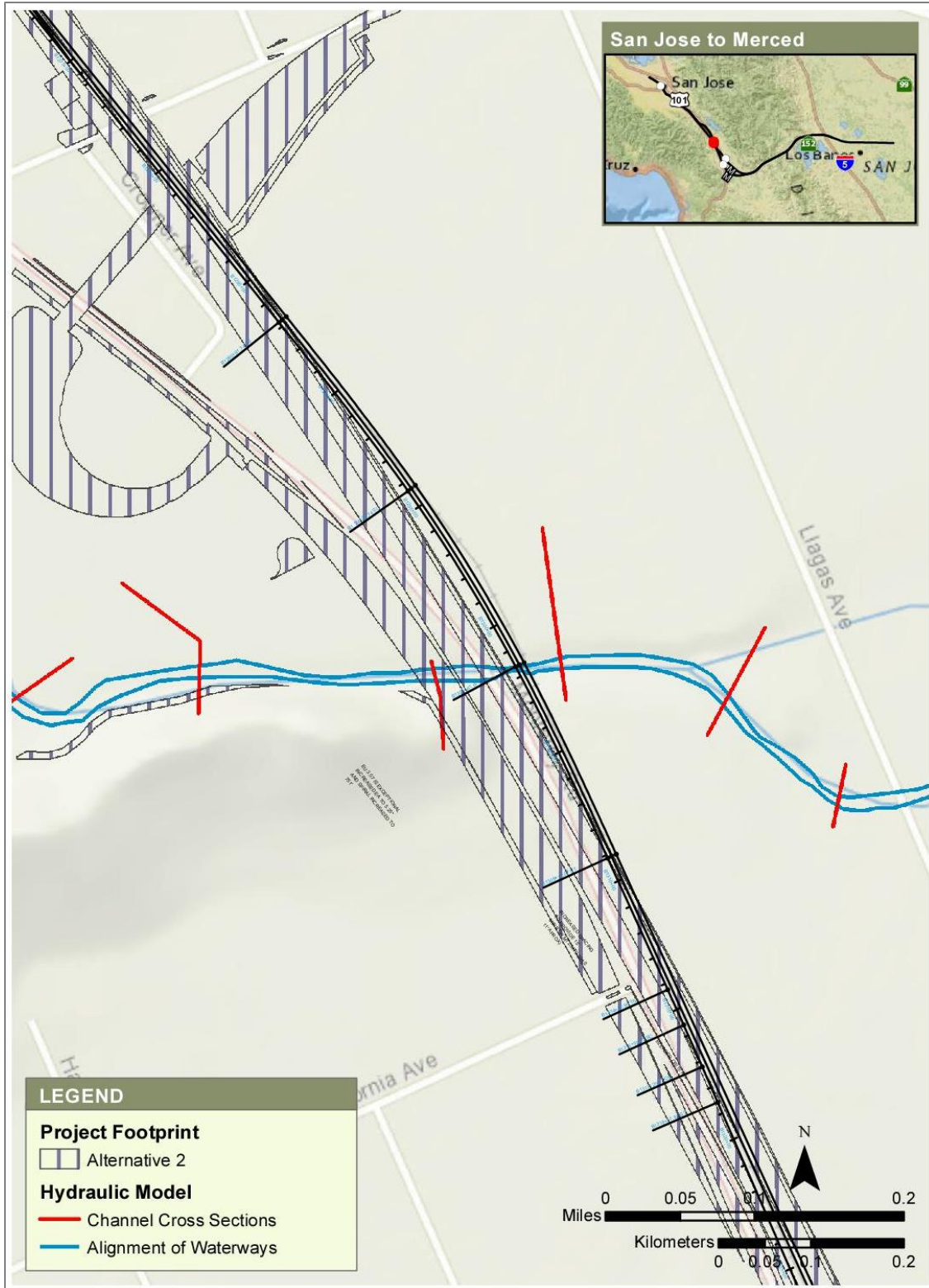
Figure 3-24 Llagas Creek (near San Martin), Plan View of FEMA Effective Hydraulic Model with Project Footprint for Alternative 2
