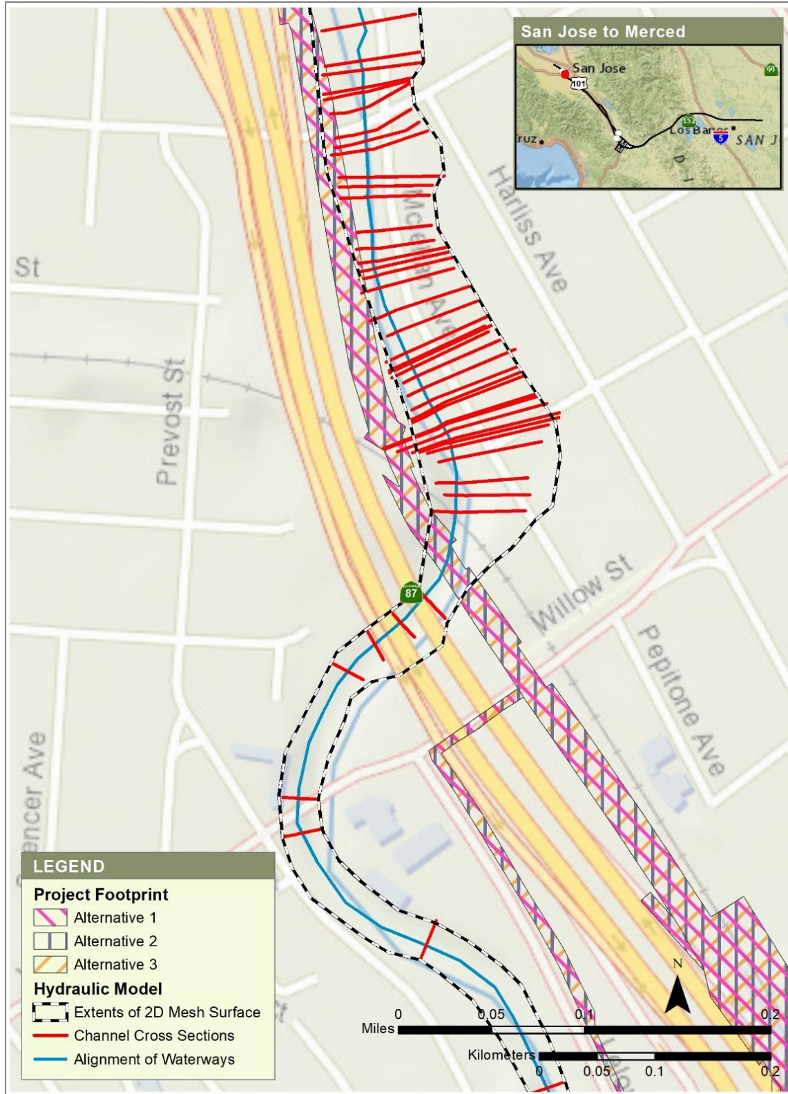
Figure 4-8 Guadalupe River, Plan View of SCVWD Hydraulic Model at Guadalupe River mainline with Project Footprints for Alternatives 1, 2, and 3
