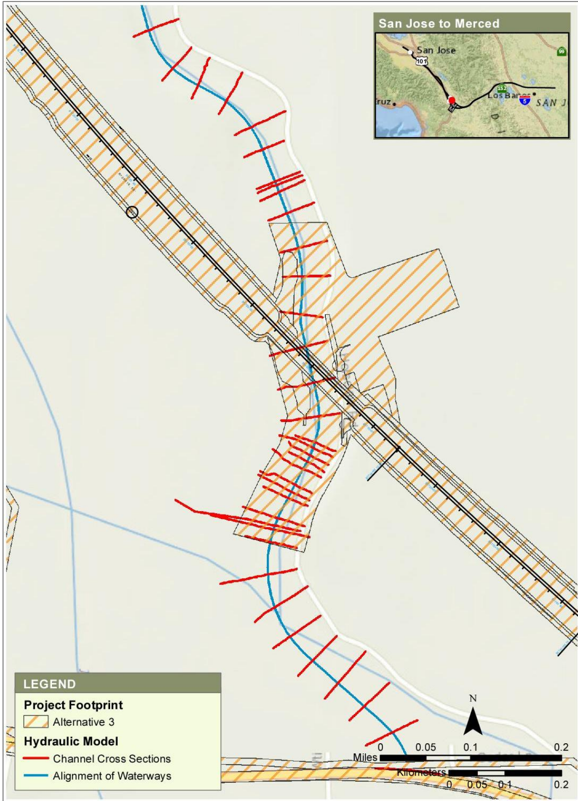
Figure 3-41 Llagas Creek (East of Gilroy), HEC-RAS Channel Cross Sections at Project Location
