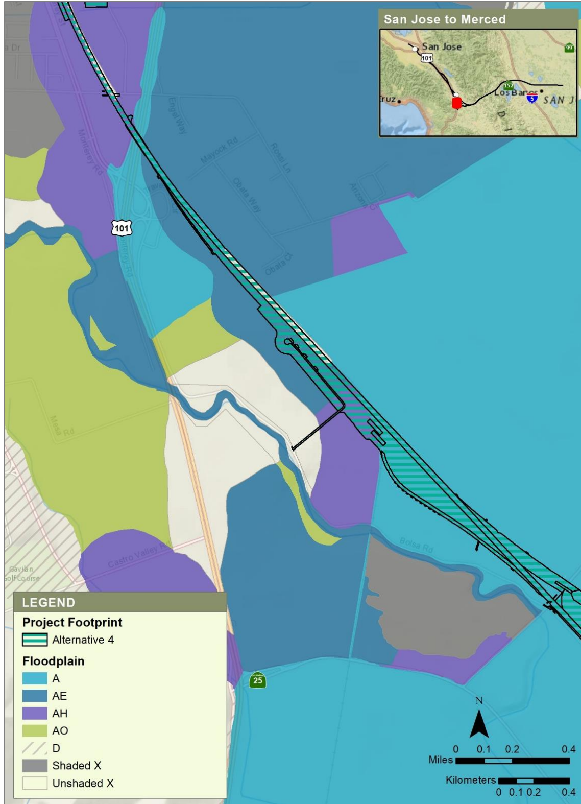
Figure 4-31 FEMA FIRM, Uvas-Carnadero Creek at Project Location with Project Footprint for Alternative 4
