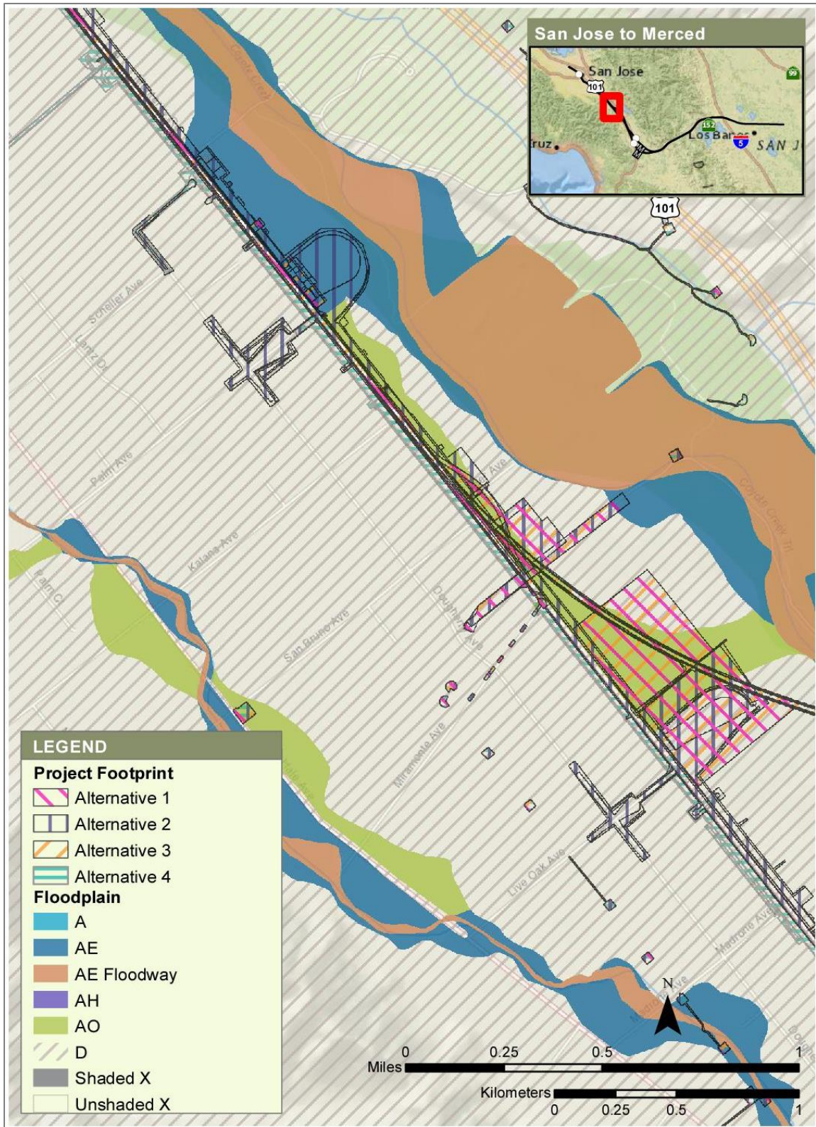
Figure 3-2 Coyote Creek, FEMA FIRM Overlay with Project Footprints for Alternatives 1, 2, 3, and 4, Page 2/2
