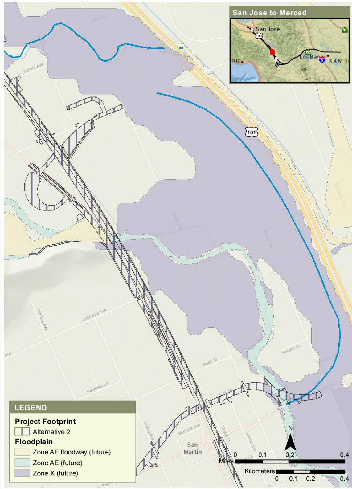
Figure 3-34 West Little Llagas Creek Middle Avenue Overflow, Floodplain after Completion of Upper Llagas Flood Protection Project with Project Footprint for Alternative 2
