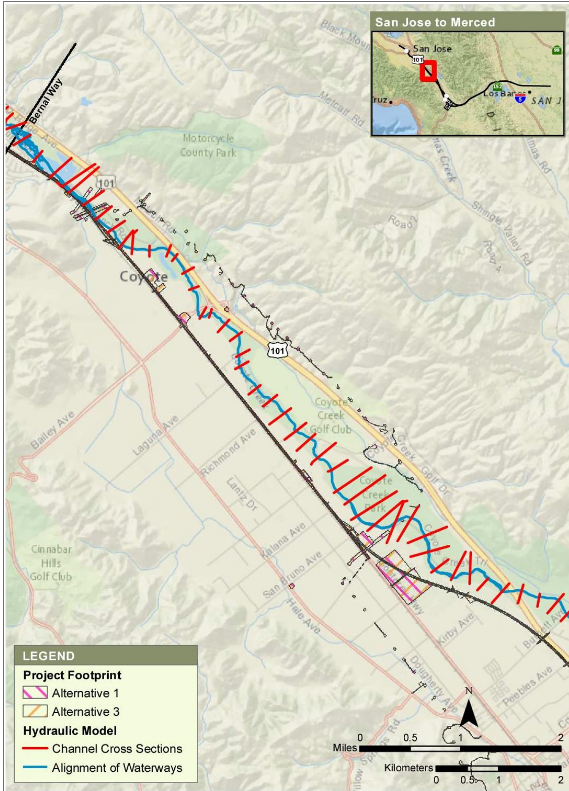
Figure 3-3 Coyote Creek, Plan View of FEMA Effective Hydraulic Model with Project Footprint for Alternatives 1 and 3
