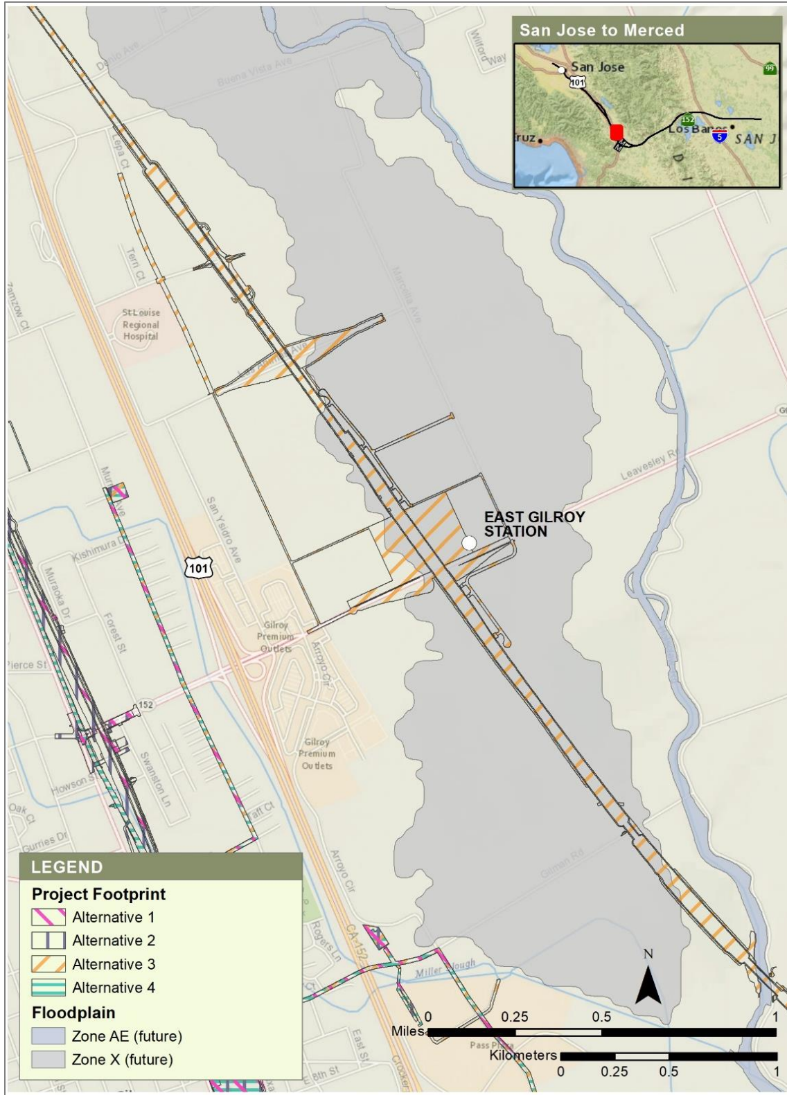
Figure 3-44 Llagas Overbank, Floodplain after Completion of Upper Llagas Flood Protection Project with Project Footprints for Alternatives 1, 2, 3, and 4
