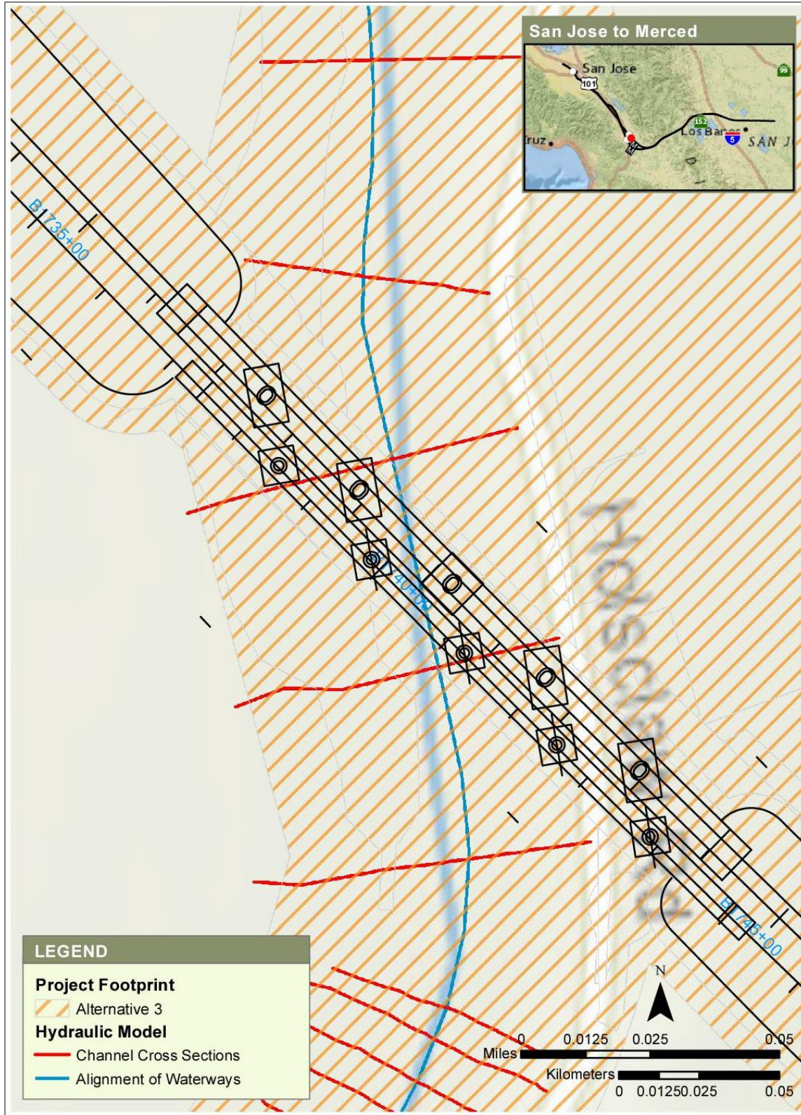
Figure 3-42 Llagas Creek (East of Gilroy), HEC-RAS Channel Cross Sections, Zoomed to Proposed Llagas Creek Bridge for Alternative 3
