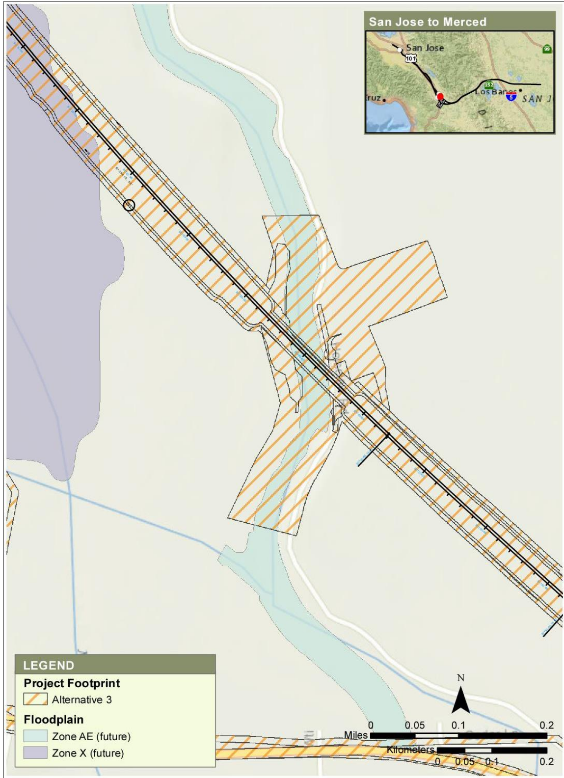
Figure 3-39 Llagas Creek (East of Gilroy), Floodplain after Completion of Upper Llagas Flood Protection Project with Project Footprint for Alternative 3
