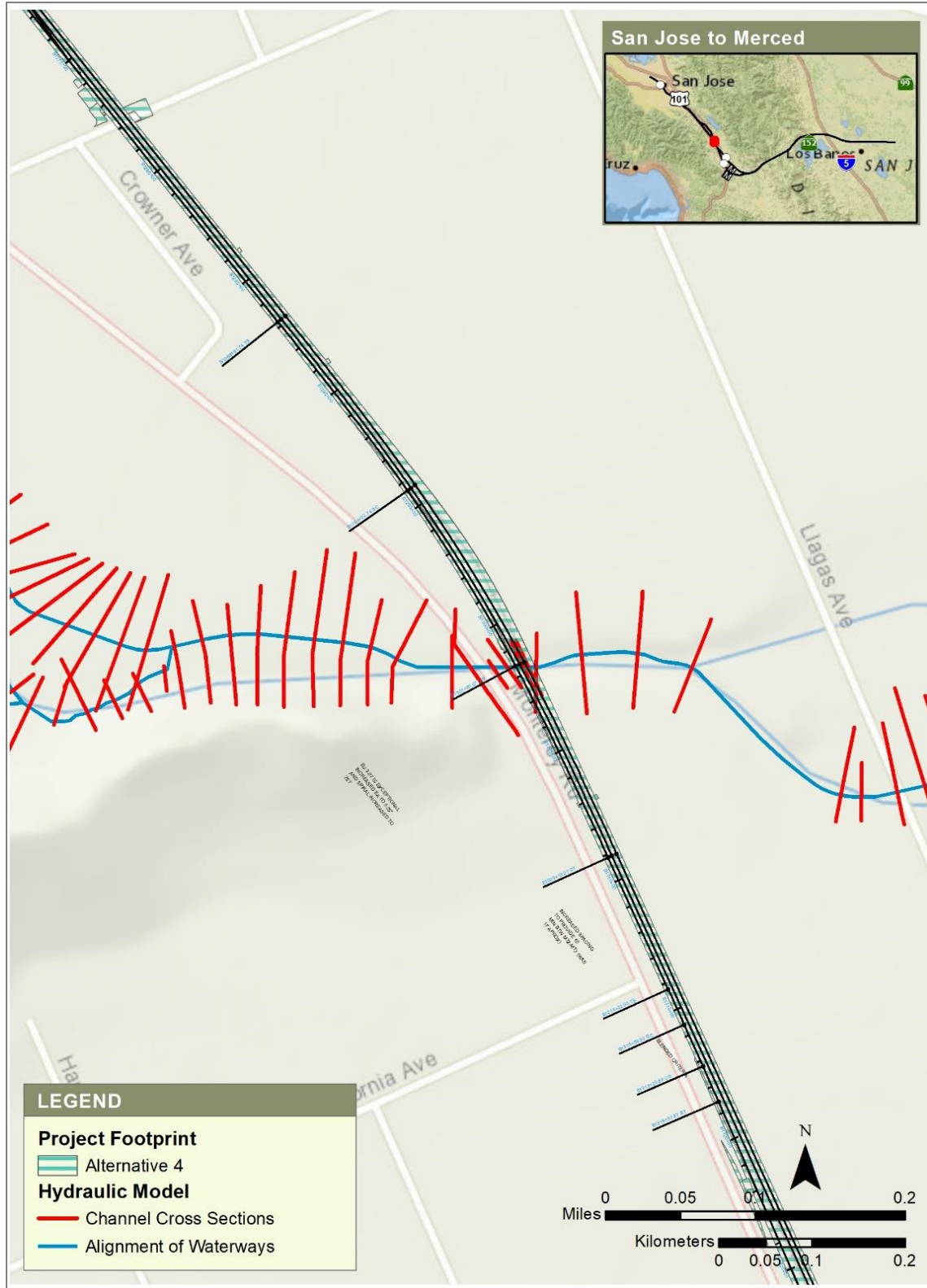
Figure 3-28 Llagas Creek (near San Martin), Plan View of SCVWD Model at Proposed HSR Crossing, Alternative 4
