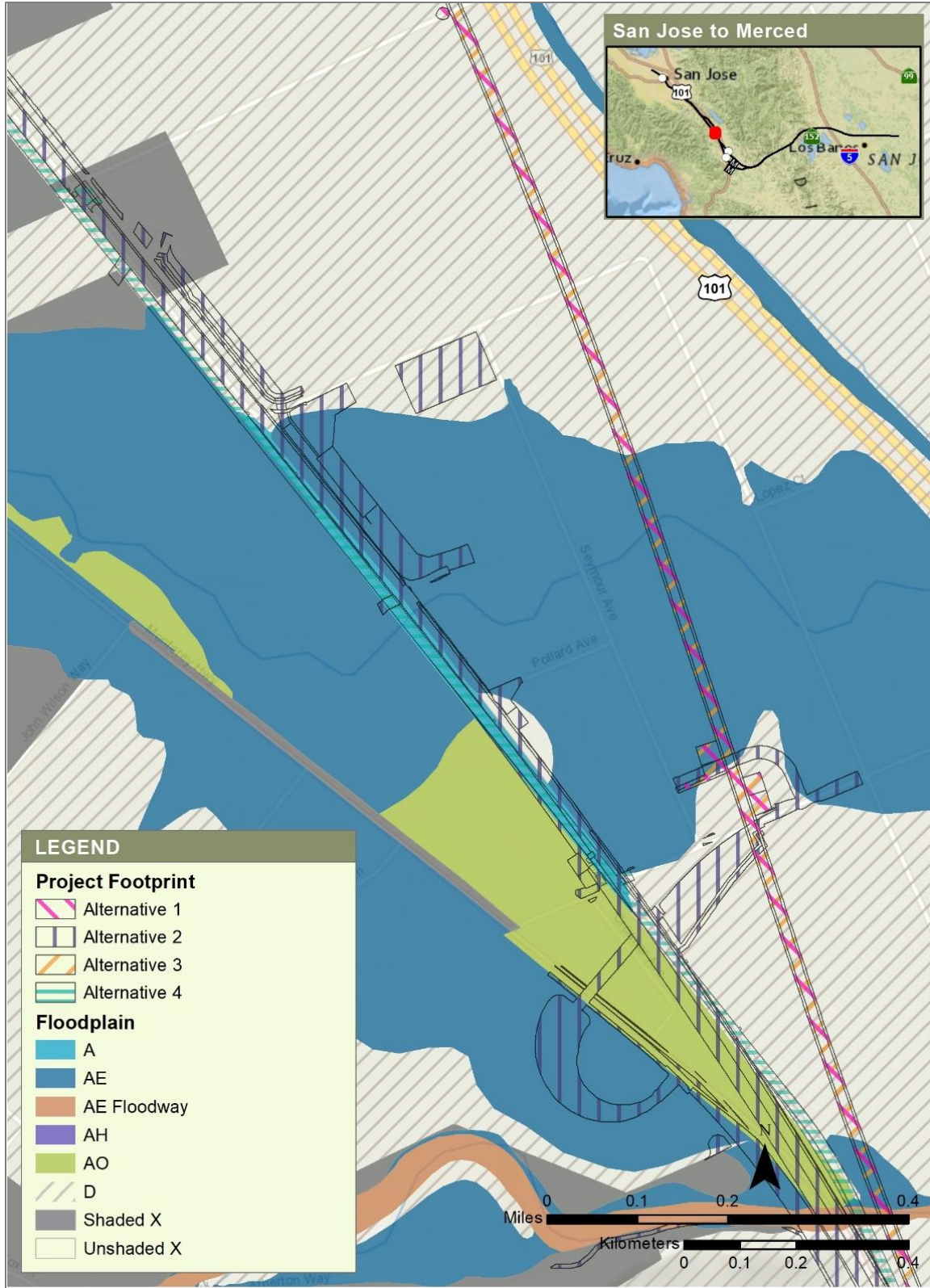
Figure 3-12 West Little Llagas Creek, FEMA FIRM Overlay with Project Footprints for Alternatives 1, 2, 3, and 4
