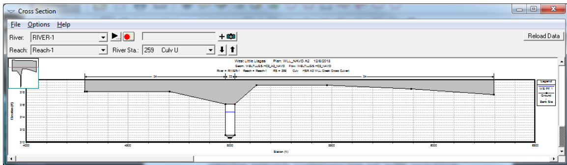
Figure 3-19 West Little Llagas Creek, HEC-RAS Channel Cross Section with Proposed Embankment Section for Alternative 2
