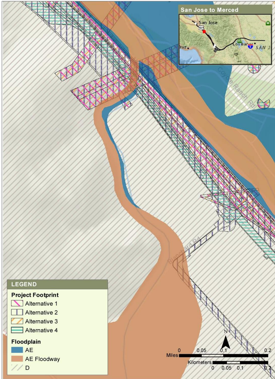
Figure 4-22 FEMA FIRM, Fisher Creek at Project Location
