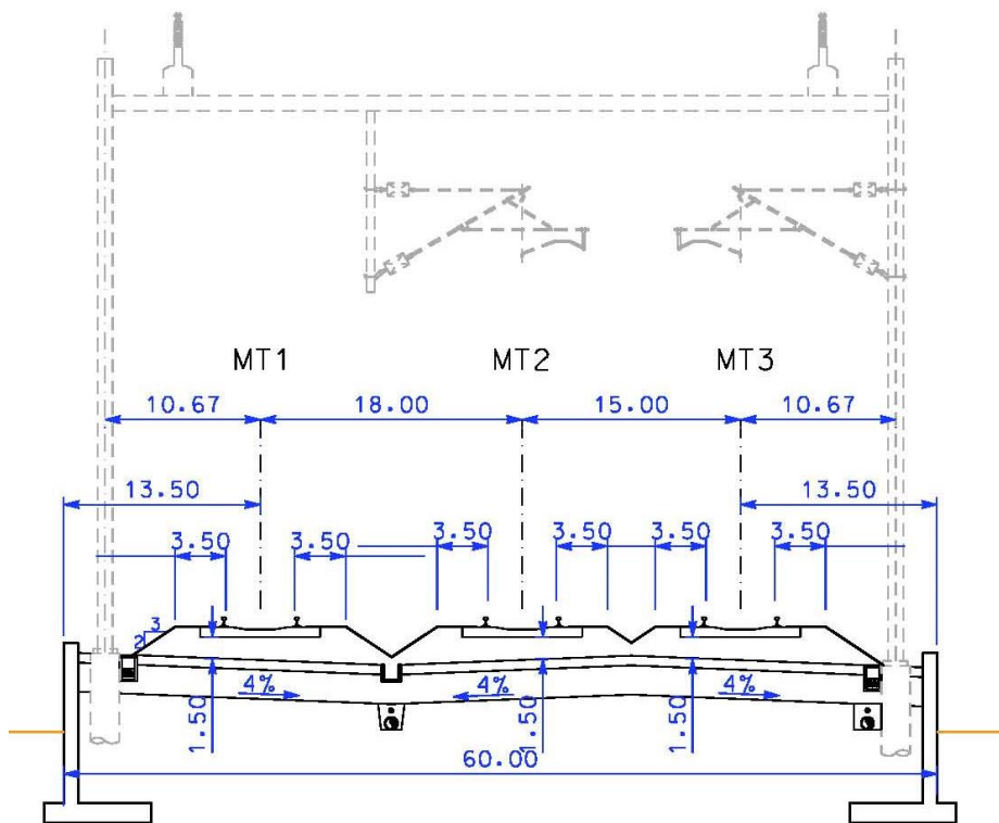
Figure 1. Typical section 60 ft.
