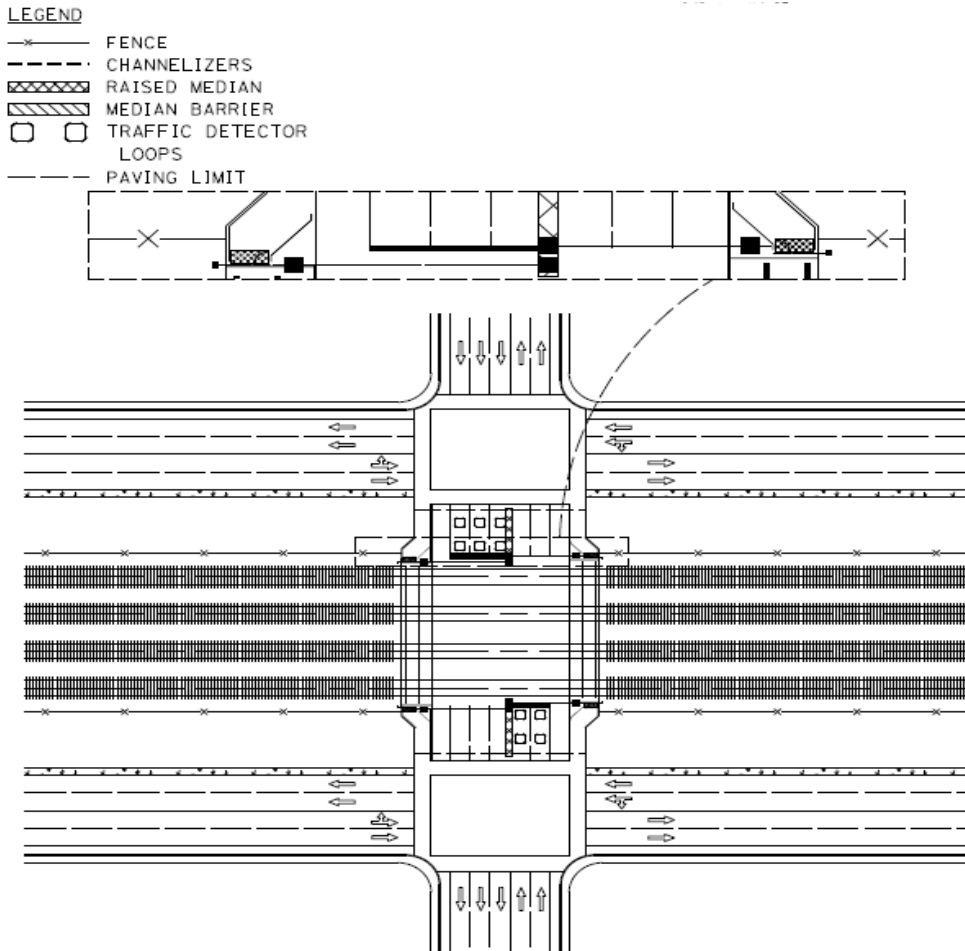
Figure 5. Scheme of grade crossing finished.
